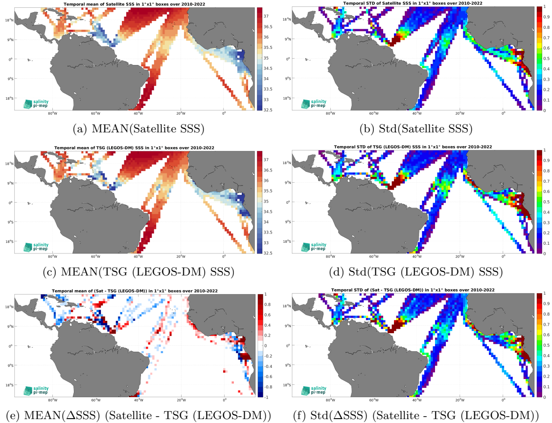
Figure 7: Temporal mean (left) and Std (right) of SSS from SMOS SSS L4 v1 - Daily (CMEMS-CNR) (top), TSG (LEGOS-DM) (middle), and of \Delta\text{SSS}(\text{Satellite} - \text{TSG}(\text{LEGOS-DM})) . Only match-up pairs are used to generate these maps.
