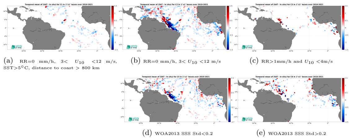
Figure 14: Temporal mean gridded over spatial boxes of size 1^\circ \times 1^\circ of \Delta\text{SSS} (SMOS SSS L4 v1 - Daily (CMEMS-CNR) - TSG (GOSUD-Research-vessel)) for 5 different subdatasets corresponding to:RR=0 mm/h, 3 < U_{10} < 12 m/s, SST >5^\circ\text{C} , distance to coast > 800 km (a), RR=0 mm/h, 3 < U_{10} < 12 m/s (b), RR >1 mm/h and U_{10} < 4 m/s (c), WOA2013 SSS Std <0.2 (d), WOA2013 SSS Std >0.2 (e).
