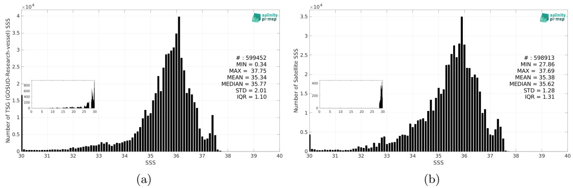
Figure 3: Histograms of SSS from TSG (GOSUD-Research-vessel) (a) and SMOS SSS L4 v1 - Daily (CMEMS-CNR) (b) considering all match-up pairs per bins of 0.1 over the Tropical Atlantic Ocean Pi-MEP region and for the full satellite product period.
