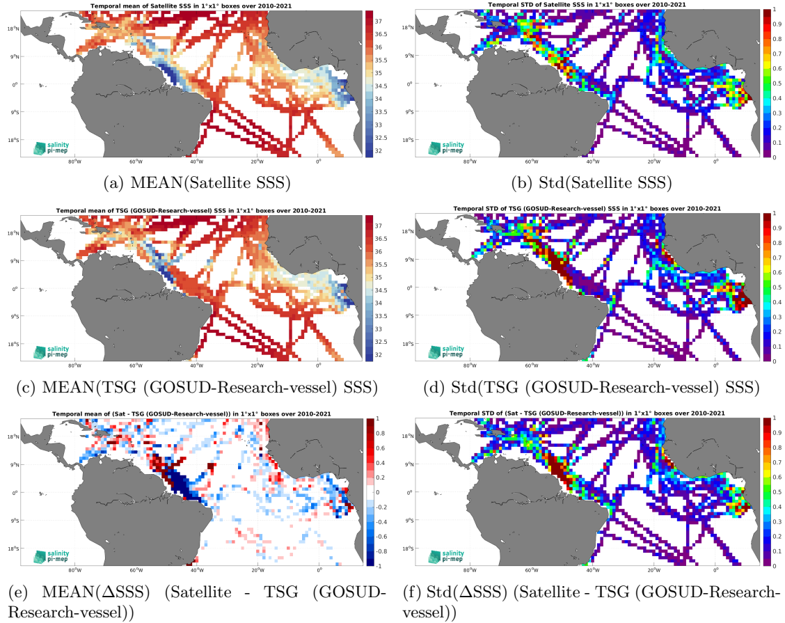
Figure 7: Temporal mean (left) and Std (right) of SSS from SMOS SSS L4 v1 - Daily (CMEMS-CNR) (top), TSG (GOSUD-Research-vessel) (middle), and of \Delta\text{SSS} (Satellite - TSG (GOSUD-Research-vessel)). Only match-up pairs are used to generate these maps.
