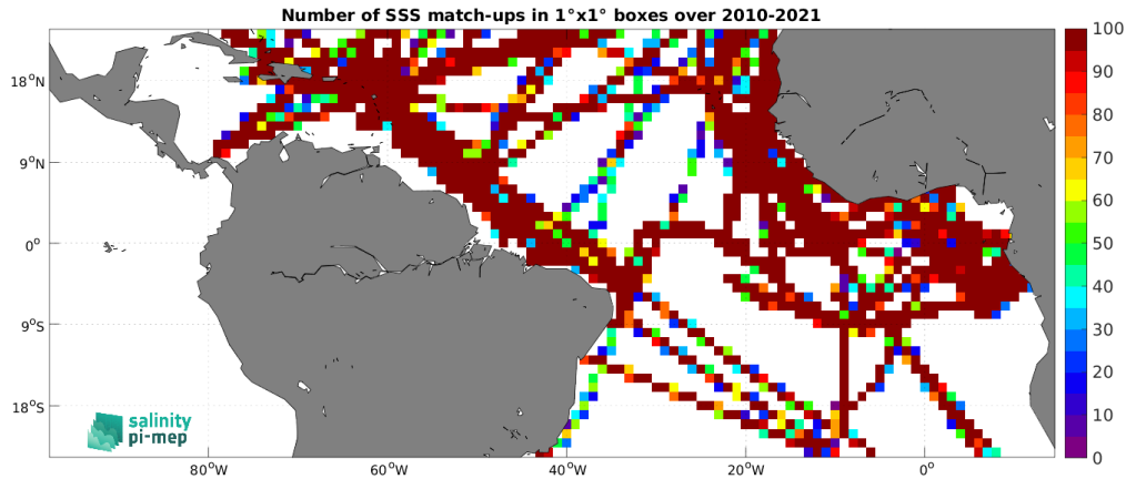
Figure 5: Number of SSS match-ups between TSG (GOSUD-Research-vessel) SSS and the SMOS SSS L4 v1 - Daily (CMEMS-CNR) SSS product for the Tropical Atlantic Ocean Pi-MEP region over 1^\circ \times 1^\circ boxes and for the full satellite product period.
