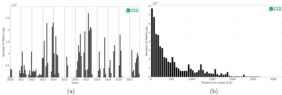
Figure 2: Number of match-ups between TSG (GOSUD-Research-vessel) and SMOS SSS L4 v1 - Daily (CMEMS-CNR) SSS as a function of time (a) and as function of the distance to coast (b) over the Tropical Atlantic Ocean Pi-MEP region and for the full satellite product period.
