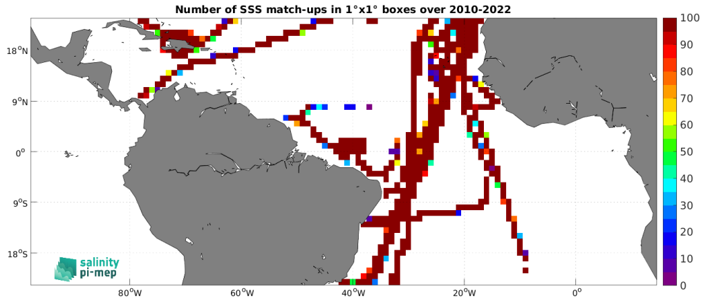
Figure 5: Number of SSS match-ups between TSG (CSIC-UTM) SSS and the SMOS SSS L4 v1 - Daily (CMEMS-CNR) SSS product for the Tropical Atlantic Ocean Pi-MEP region over 1^\circ \times 1^\circ boxes and for the full satellite product period.
