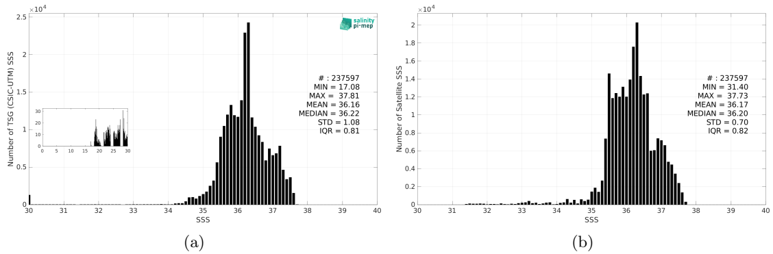
Figure 3: Histograms of SSS from TSG (CSIC-UTM) (a) and SMOS SSS L4 v1 - Daily (CMEMS-CNR) (b) considering all match-up pairs per bins of 0.1 over the Tropical Atlantic Ocean Pi-MEP region and for the full satellite product period.
