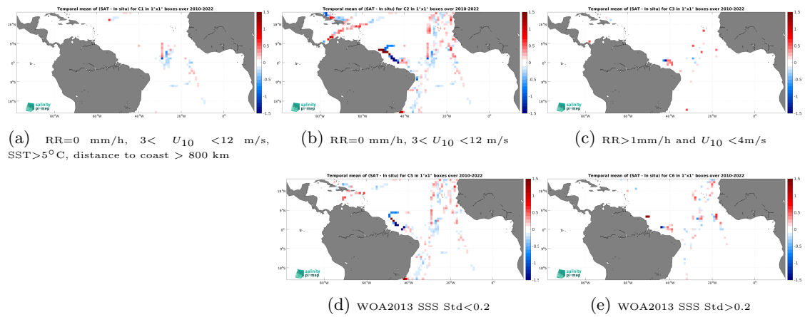
Figure 14: Temporal mean gridded over spatial boxes of size 1^\circ \times 1^\circ of \Delta SSS (SMOS SSS L4 v1 - Daily (CMEMS-CNR) - TSG (CSIC-UTM)) for 5 different subdatasets corresponding to:RR=0 mm/h, 3 < U_{10} < 12 m/s, SST>5°C, distance to coast > 800 km (a), RR=0 mm/h, 3 < U_{10} < 12 m/s (b), RR>1mm/h and U_{10} < 4 m/s (c), WOA2013 SSS Std<0.2 (d), WOA2013 SSS Std>0.2 (e).
