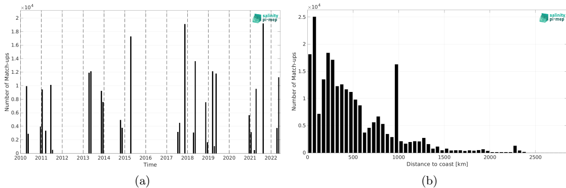
Figure 2: Number of match-ups between TSG (CSIC-UTM) and SMOS SSS L4 v1 - Daily (CMEMS-CNR) SSS as a function of time (a) and as function of the distance to coast (b) over the Tropical Atlantic Ocean Pi-MEP region and for the full satellite product period.
