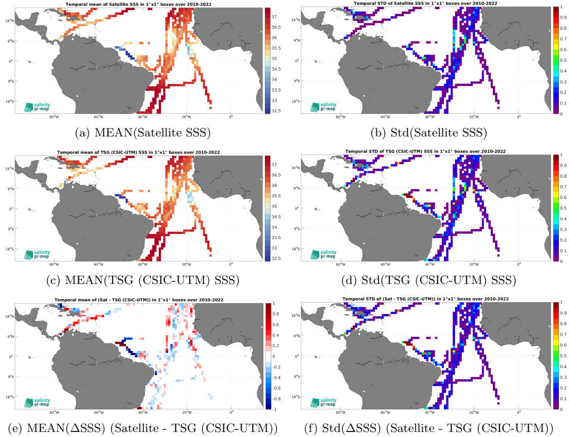
Figure 7: Temporal mean (left) and Std (right) of SSS from SMOS SSS L4 v1 - Daily (CMEMS-CNR) (top), TSG (CSIC-UTM) (middle), and of \Delta\text{SSS} (Satellite - TSG (CSIC-UTM)). Only match-up pairs are used to generate these maps.
