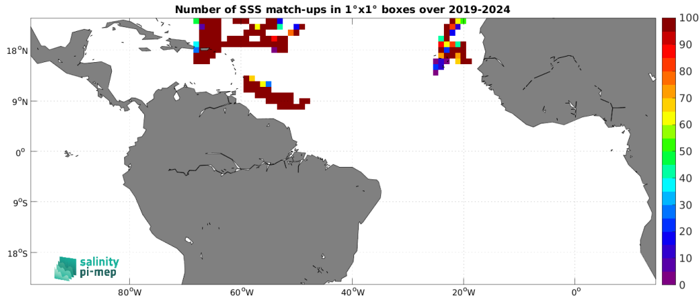
Figure 5: Number of SSS match-ups between Saildrone SSS and the SMOS SSS L4 v1 - Daily (CMEMS-CNR) SSS product for the Tropical Atlantic Ocean Pi-MEP region over 1^\circ \times 1^\circ boxes and for the full satellite product period.
