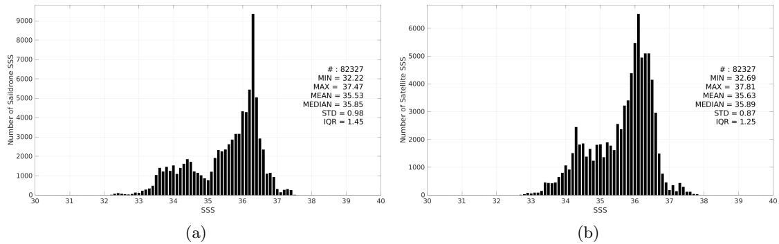
Figure 3: Histograms of SSS from Saildrone (a) and SMOS SSS L4 v1 - Daily (CMEMS-CNR) (b) considering all match-up pairs per bins of 0.1 over the Tropical Atlantic Ocean Pi-MEP region and for the full satellite product period.
