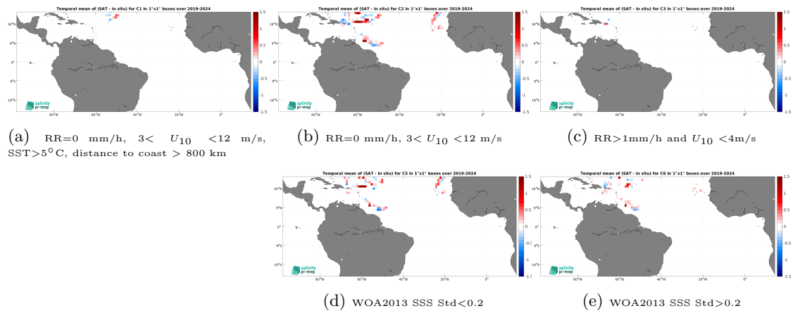
Figure 14: Temporal mean gridded over spatial boxes of size 1^\circ \times 1^\circ of \Delta\text{SSS} (SMOS SSS L4 v1 - Daily (CMEMS-CNR) - Sailability) for 5 different subdatasets corresponding to:RR=0 mm/h, 3 < U_{10} < 12 m/s, SST >5^\circ\text{C} , distance to coast > 800 km (a), RR=0 mm/h, 3 < U_{10} < 12 m/s (b), RR >1 mm/h and U_{10} < 4 m/s (c), WOA2013 SSS Std <0.2 (d), WOA2013 SSS Std >0.2 (e).
