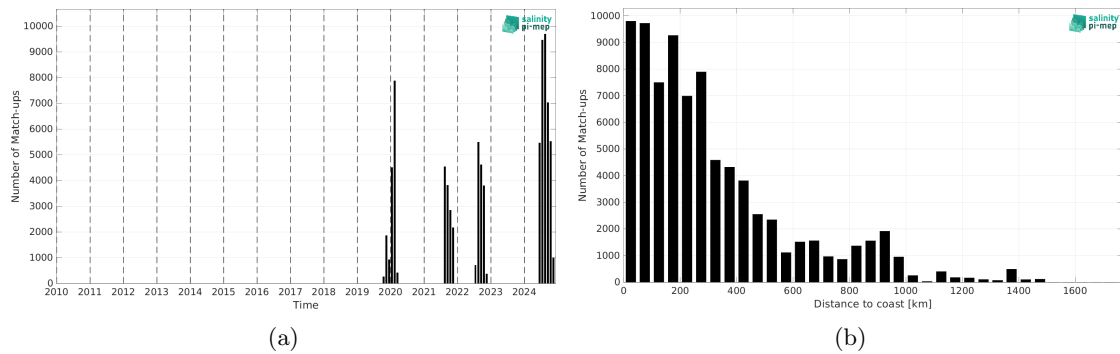
Figure 2: Number of match-ups between Saildrone and SMOS SSS L4 v1 - Daily (CMEMS-CNR) SSS as a function of time (a) and as function of the distance to coast (b) over the Tropical Atlantic Ocean Pi-MEP region and for the full satellite product period.
