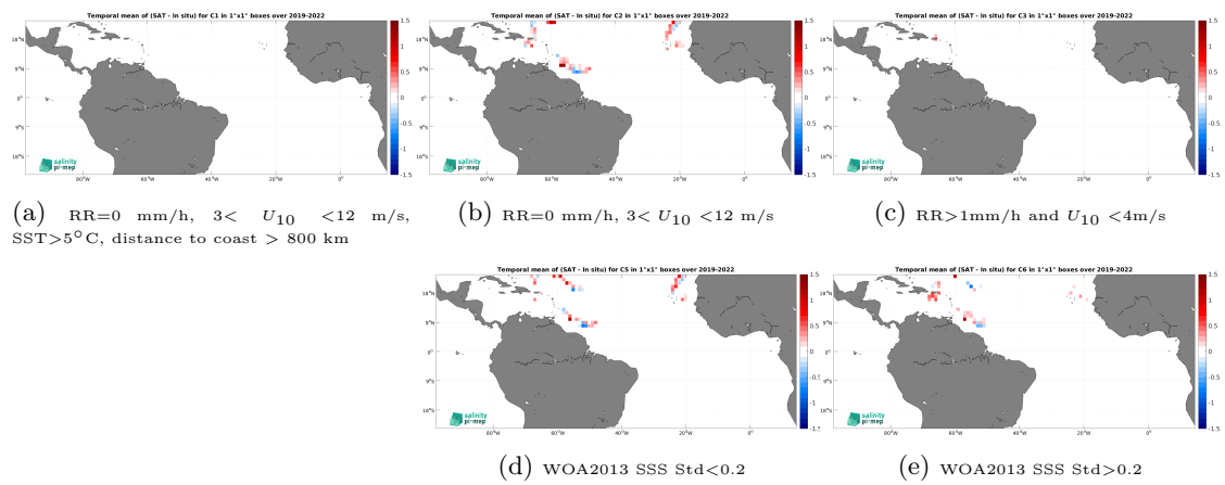
Figure 14: Temporal mean gridded over spatial boxes of size 1^\circ \times 1^\circ of \Delta SSS (SMOS SSS L4 v1 - Daily (CMEMS-CNR) - Sailability) for 5 different subdatasets corresponding to:RR=0 mm/h, 3 < U_{10} < 12 m/s, SST >5^\circ\text{C} , distance to coast > 800 km (a), RR=0 mm/h, 3 < U_{10} < 12 m/s (b), RR >1 mm/h and U_{10} < 4 m/s (c), WOA2013 SSS Std <0.2 (d), WOA2013 SSS Std >0.2 (e).
