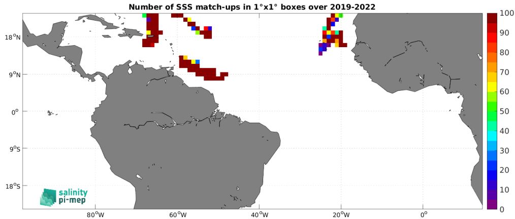
Figure 5: Number of SSS match-ups between Saildrone SSS and the SMOS SSS L4 v1 - Daily (CMEMS-CNR) SSS product for the Tropical Atlantic Ocean Pi-MEP region over 1^{\circ} \times 1^{\circ} boxes and for the full satellite product period.
