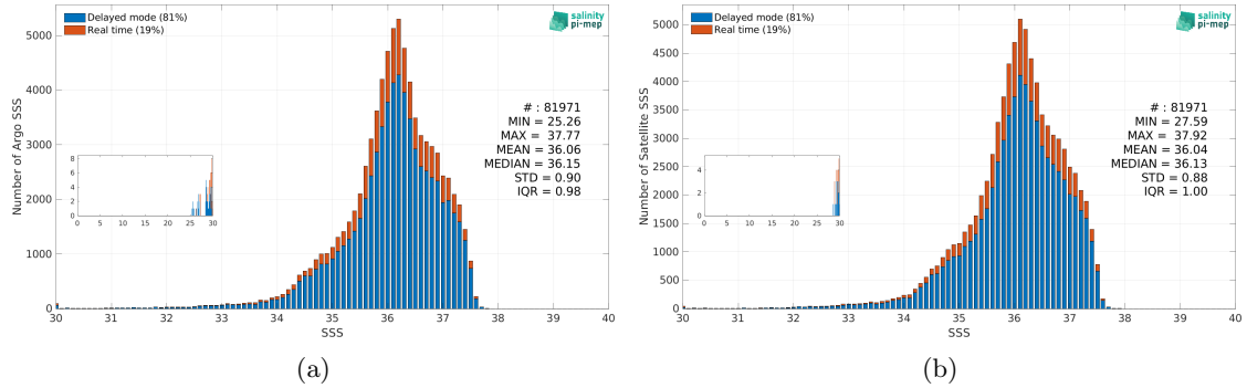
Figure 3: Histograms of SSS from Argo (a) and SMOS SSS L4 v1 - Daily (CMEMS-CNR) (b) considering all match-up pairs per bins of 0.1 over the Tropical Atlantic Ocean Pi-MEP region and for the full satellite product period.
