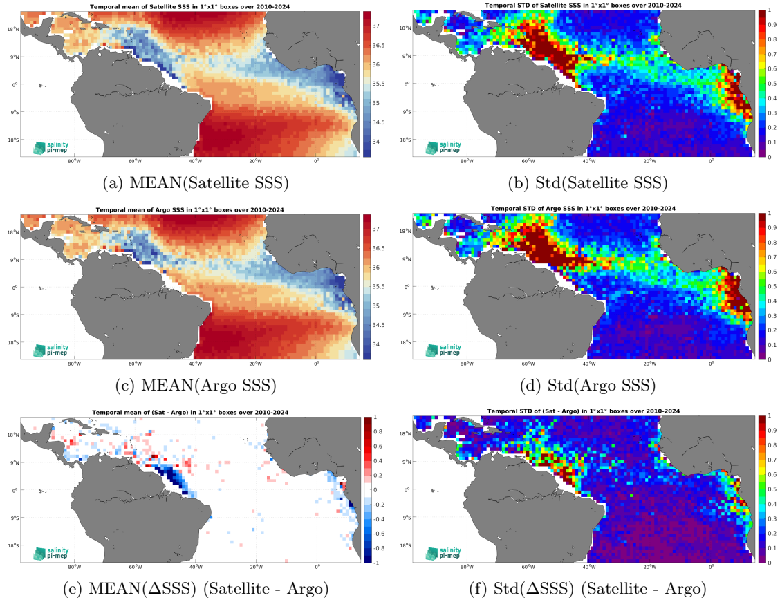
Figure 7: Temporal mean (left) and Std (right) of SSS from SMOS SSS L4 v1 - Daily (CMEMS-CNR) (top), Argo (middle), and of \Delta\text{SSS} (Satellite - Argo). Only match-up pairs are used to generate these maps.
