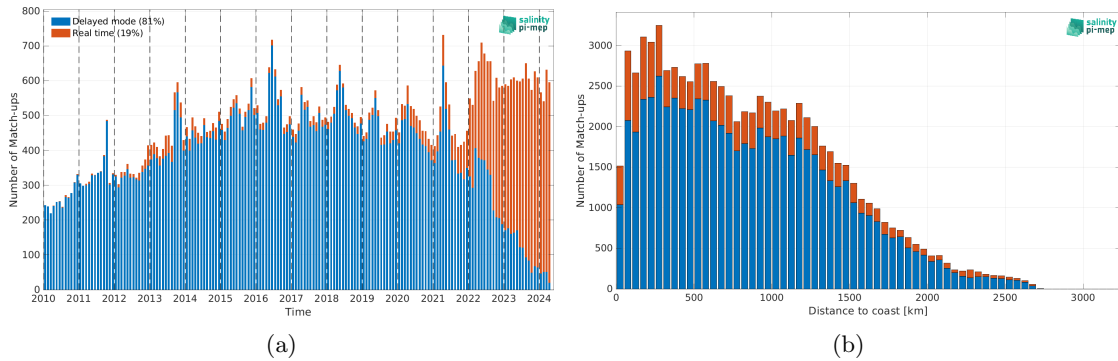
Figure 2: Number of match-ups between Argo and SMOS SSS L4 v1 - Daily (CMEMS-CNR) SSS as a function of time (a) and as function of the distance to coast (b) over the Tropical Atlantic Ocean Pi-MEP region and for the full satellite product period.
