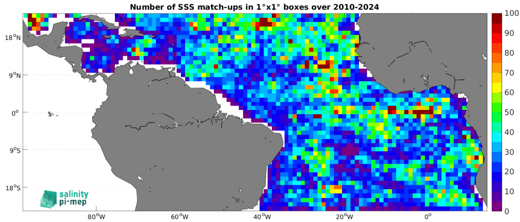
Figure 5: Number of SSS match-ups between Argo SSS and the SMOS SSS L4 v1 - Daily (CMEMS-CNR) SSS product for the Tropical Atlantic Ocean Pi-MEP region over 1^\circ \times 1^\circ boxes and for the full satellite product period.
