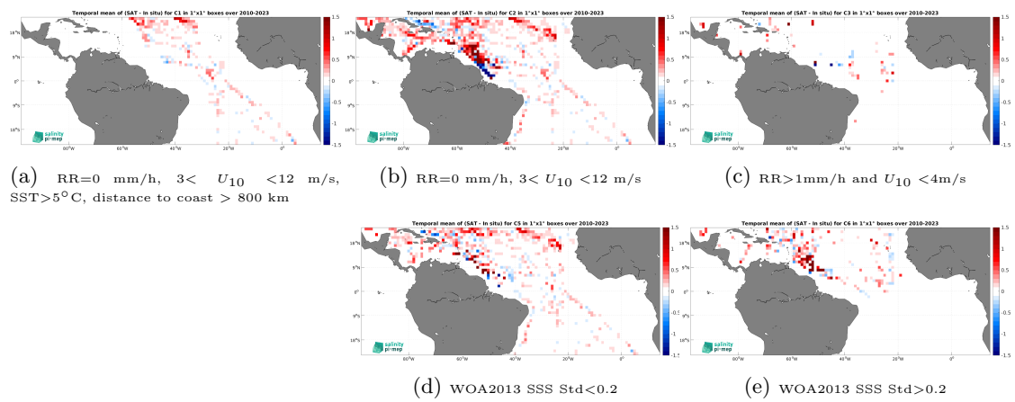
Figure 14: Temporal mean gridded over spatial boxes of size 1^\circ \times 1^\circ of \Delta\text{SSS} (SMOS SSS L4 OI v346 - Weekly (CMEMS-CATDS-LOPS) - TSG (SAMOS)) for 5 different subdatasets corresponding to:RR=0 mm/h, 3 < U_{10} < 12 m/s, SST >5^\circ\text{C} , distance to coast > 800 km (a), RR=0 mm/h, 3 < U_{10} < 12 m/s (b), RR >1 mm/h and U_{10} < 4 m/s (c), WOA2013 SSS Std <0.2 (d), WOA2013 SSS Std >0.2 (e).
