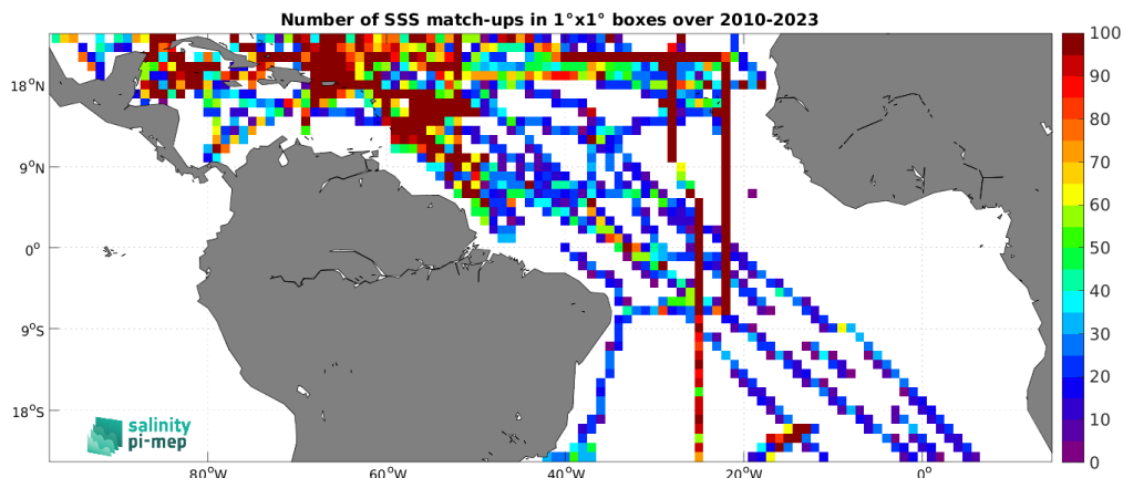
Figure 5: Number of SSS match-ups between TSG (SAMOS) SSS and the SMOS SSS L4 OI v346 - Weekly (CMEMS-CATDS-LOPS) SSS product for the Tropical Atlantic Ocean Pi-MEP region over 1^\circ \times 1^\circ boxes and for the full satellite product period.
