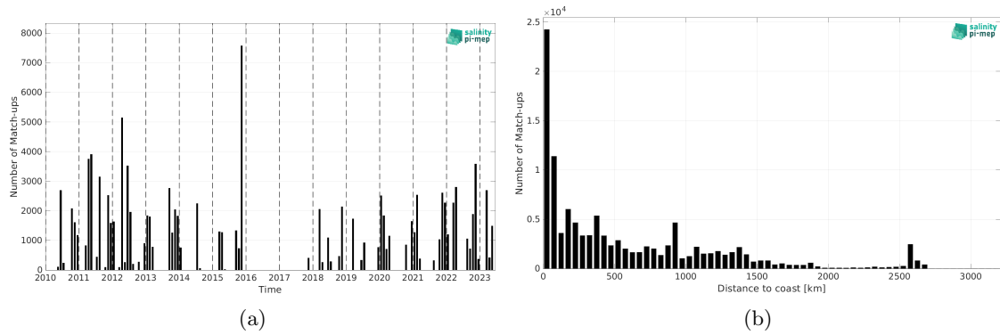
Figure 2: Number of match-ups between TSG (SAMOS) and SMOS SSS L4 OI v346 - Weekly (CMEMS-CATDS-LOPS) SSS as a function of time (a) and as function of the distance to coast (b) over the Tropical Atlantic Ocean Pi-MEP region and for the full satellite product period.
