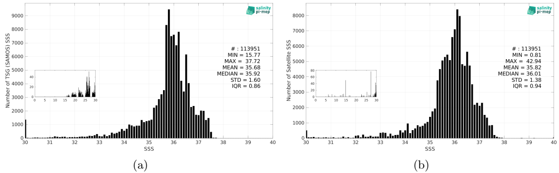
Figure 3: Histograms of SSS from TSG (SAMOS) (a) and SMOS SSS L4 OI v346 - Weekly (CMEMS-CATDS-LOPS) (b) considering all match-up pairs per bins of 0.1 over the Tropical Atlantic Ocean Pi-MEP region and for the full satellite product period.
