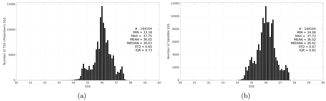
Figure 3: Histograms of SSS from TSG (Polarstern) (a) and SMOS SSS L4 OI v346 - Weekly (CMEMS-CATDS-LOPS) (b) considering all match-up pairs per bins of 0.1 over the Tropical Atlantic Ocean Pi-MEP region and for the full satellite product period.
