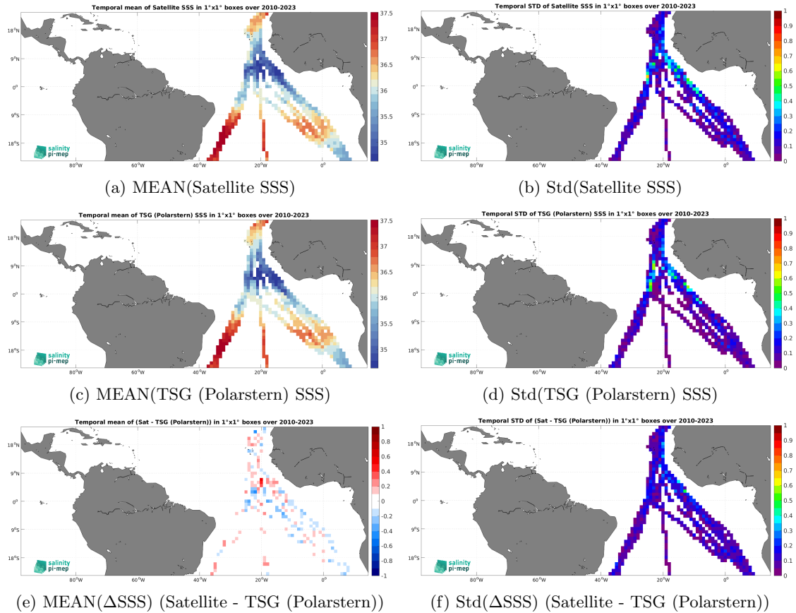
Figure 7: Temporal mean (left) and Std (right) of SSS from SMOS SSS L4 OI v346 - Weekly (CMEMS-CATDS-LOPS) (top), TSG (Polarstern) (middle), and of \Delta SSS (Satellite - TSG (Polarstern)). Only match-up pairs are used to generate these maps.
