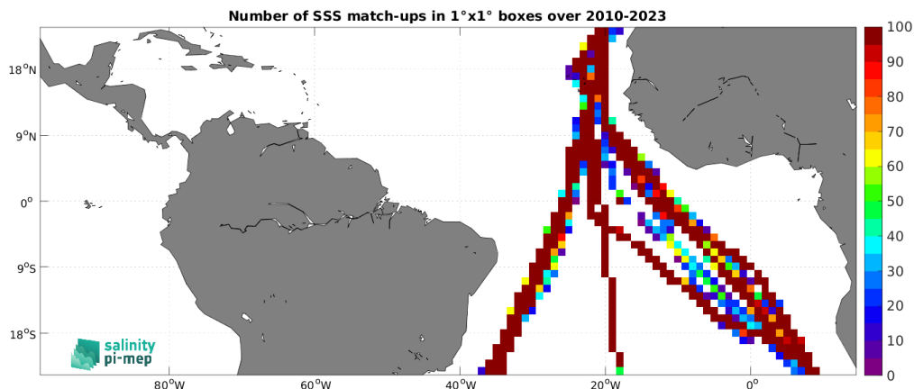
Figure 5: Number of SSS match-ups between TSG (Polarstern) SSS and the SMOS SSS L4 OI v346 - Weekly (CMEMS-CATDS-LOPS) SSS product for the Tropical Atlantic Ocean Pi-MEP region over 1^\circ \times 1^\circ boxes and for the full satellite product period.
