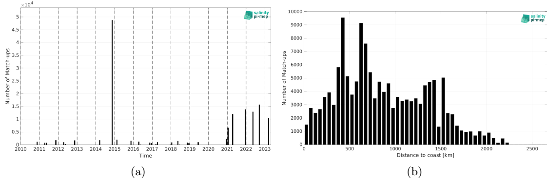
Figure 2: Number of match-ups between TSG (Polarstern) and SMOS SSS L4 OI v346 - Weekly (CMEMS-CATDS-LOPS) SSS as a function of time (a) and as function of the distance to coast (b) over the Tropical Atlantic Ocean Pi-MEP region and for the full satellite product period.
