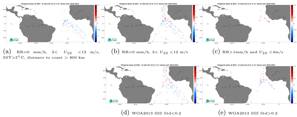
Figure 14: Temporal mean gridded over spatial boxes of size 1^\circ \times 1^\circ of \Delta\text{SSS} (SMOS SSS L4 OI v346 - Weekly (CMEMS-CATDS-LOPS) - TSG (Polarstern)) for 5 different subdatasets corresponding to:RR=0 mm/h, 3 < U_{10} < 12 m/s, SST >5^\circ\text{C} , distance to coast > 800 km (a), RR=0 mm/h, 3 < U_{10} < 12 m/s (b), RR >1 mm/h and U_{10} < 4 m/s (c), WOA2013 SSS Std <0.2 (d), WOA2013 SSS Std >0.2 (e).
