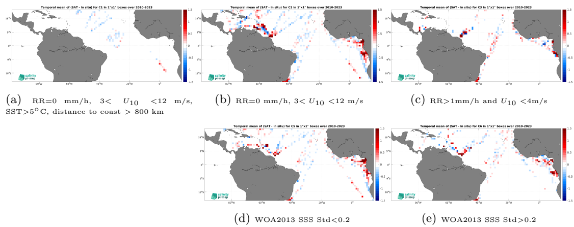
Figure 14: Temporal mean gridded over spatial boxes of size 1^\circ \times 1^\circ of \Delta\text{SSS} (SMOS SSS L4 OI v346 - Weekly (CMEMS-CATDS-LOPS) - TSG (LEGOS-DM)) for 5 different subdatasets corresponding to:RR=0 mm/h, 3 < U_{10} < 12 m/s, SST >5^\circ\text{C} , distance to coast > 800 km (a), RR=0 mm/h, 3 < U_{10} < 12 m/s (b), RR >1 mm/h and U_{10} < 4 m/s (c), WOA2013 SSS Std <0.2 (d), WOA2013 SSS Std >0.2 (e).
