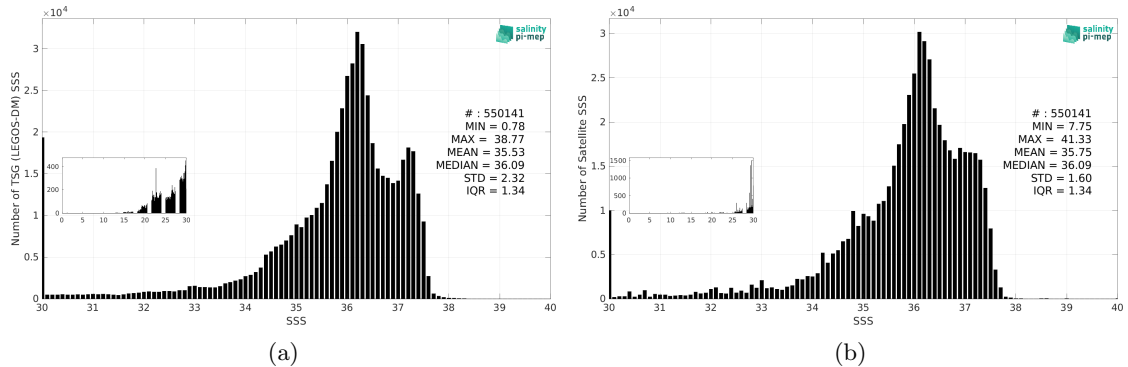
Figure 3: Histograms of SSS from TSG (LEGOS-DM) (a) and SMOS SSS L4 OI v346 - Weekly (CMEMS-CATDS-LOPS) (b) considering all match-up pairs per bins of 0.1 over the Tropical Atlantic Ocean Pi-MEP region and for the full satellite product period.
