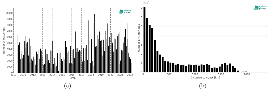
Figure 2: Number of match-ups between TSG (LEGOS-DM) and SMOS SSS L4 OI v346 - Weekly (CMEMS-CATDS-LOPS) SSS as a function of time (a) and as function of the distance to coast (b) over the Tropical Atlantic Ocean Pi-MEP region and for the full satellite product period.
