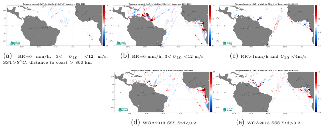
Figure 14: Temporal mean gridded over spatial boxes of size 1^\circ \times 1^\circ of \Delta SSS (SMOS SSS L4 OI v346 - Weekly (CMEMS-CATDS-LOPS) - TSG (LEGOS-DM)) for 5 different subdatasets corresponding to:RR=0 mm/h, 3 < U_{10} < 12 m/s, SST >5^\circ\text{C} , distance to coast > 800 km (a), RR=0 mm/h, 3 < U_{10} < 12 m/s (b), RR >1 mm/h and U_{10} < 4 m/s (c), WOA2013 SSS Std <0.2 (d), WOA2013 SSS Std >0.2 (e).
