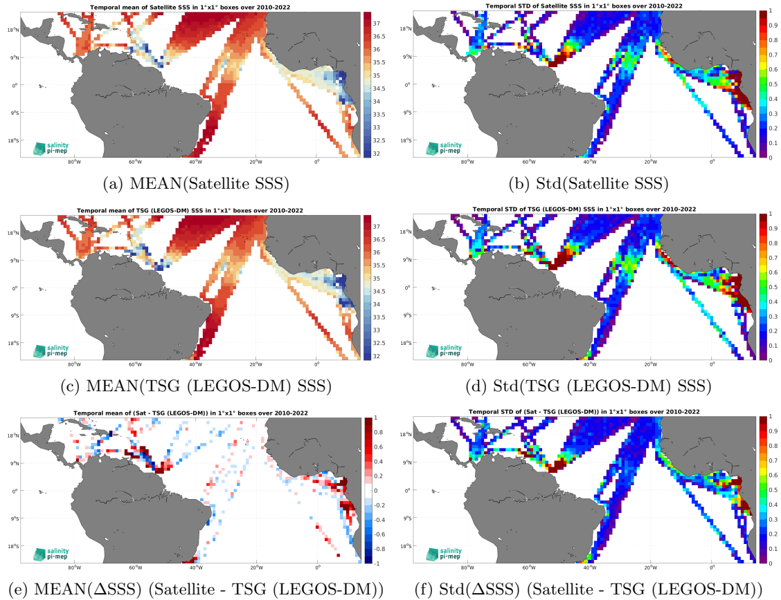
Figure 7: Temporal mean (left) and Std (right) of SSS from SMOS SSS L4 OI v346 - Weekly (CMEMS-CATDS-LOPS) (top), TSG (LEGOS-DM) (middle), and of \Delta SSS (Satellite - TSG (LEGOS-DM)). Only match-up pairs are used to generate these maps.
