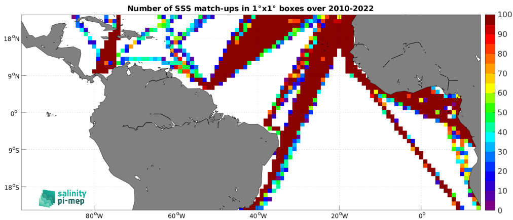
Figure 5: Number of SSS match-ups between TSG (LEGOS-DM) SSS and the SMOS SSS L4 OI v346 - Weekly (CMEMS-CATDS-LOPS) SSS product for the Tropical Atlantic Ocean Pi-MEP region over 1^\circ \times 1^\circ boxes and for the full satellite product period.
