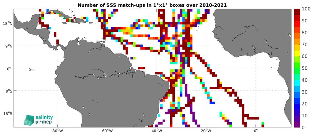
Figure 5: Number of SSS match-ups between TSG (GOSUD-Sailing-ship) SSS and the SMOS SSS L4 OI v346 - Weekly (CMEMS-CATDS-LOPS) SSS product for the Tropical Atlantic Ocean Pi-MEP region over 1^\circ \times 1^\circ boxes and for the full satellite product period.
