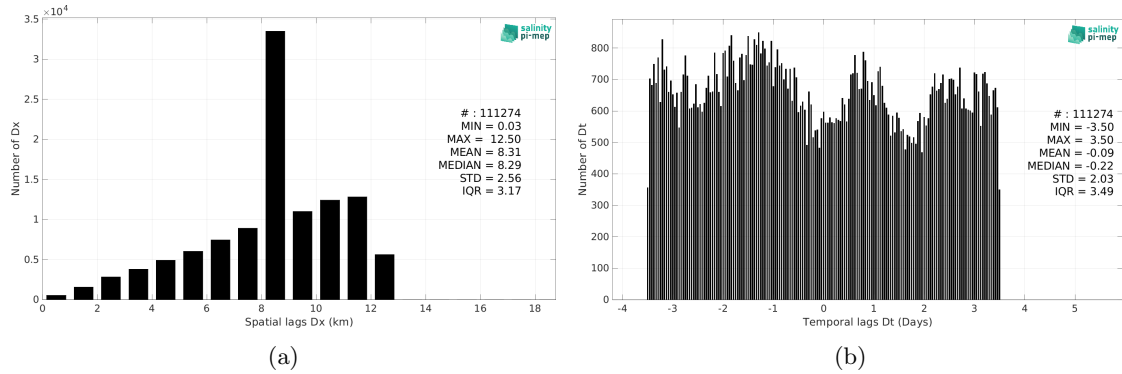
Figure 6: Histograms of the spatial (a) and temporal (b) lags between the location/time of the TSG (GOSUD-Sailing-ship) measurement and the date of the corresponding SMOS SSS L4 OI v346 - Weekly (CMEMS-CATDS-LOPS) SSS pixel.
