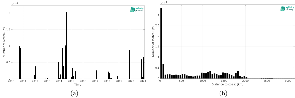
Figure 2: Number of match-ups between TSG (GOSUD-Sailing-ship) and SMOS SSS L4 OI v346 - Weekly (CMEMS-CATDS-LOPS) SSS as a function of time (a) and as function of the distance to coast (b) over the Tropical Atlantic Ocean Pi-MEP region and for the full satellite product period.
