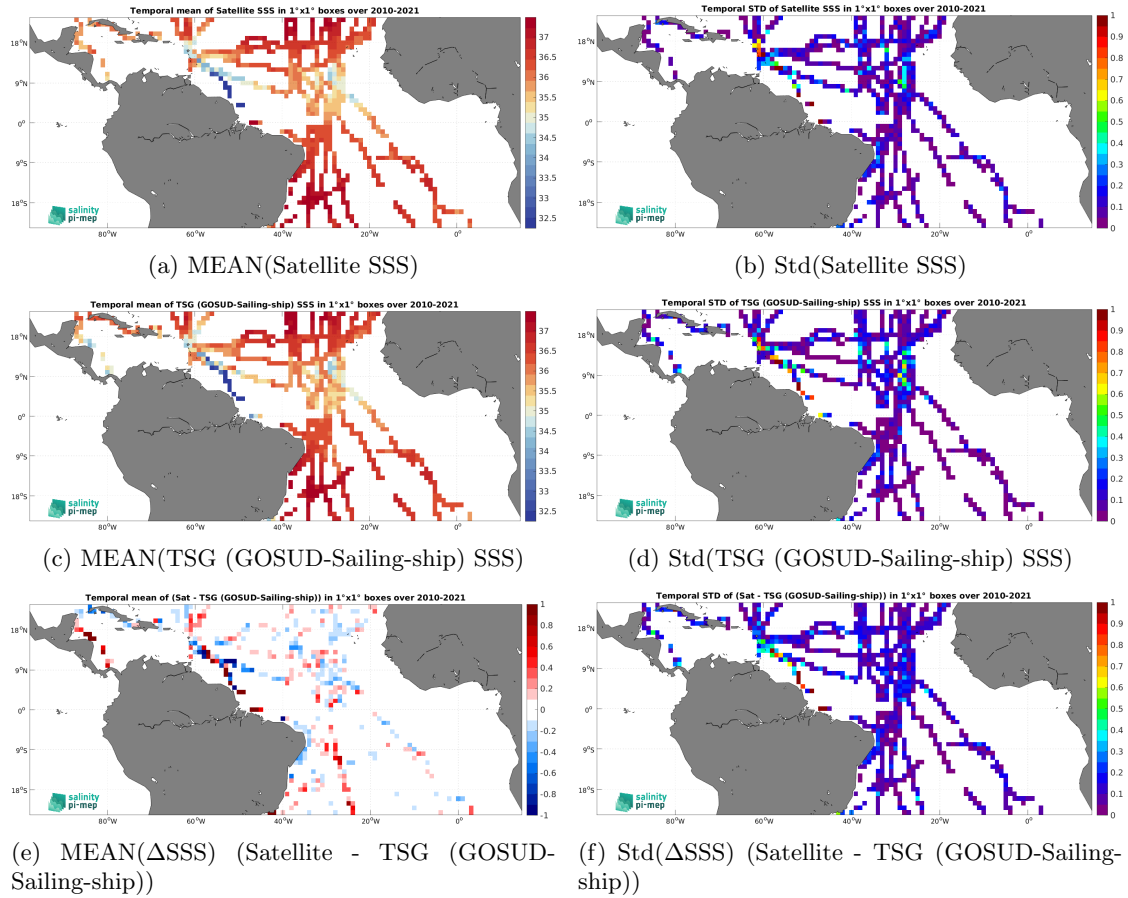
Figure 7: Temporal mean (left) and Std (right) of SSS from SMOS SSS L4 OI v346 - Weekly (CMEMS-CATDS-LOPS) (top), TSG (GOSUD-Sailing-ship) (middle), and of \Delta SSS (Satellite - TSG (GOSUD-Sailing-ship)). Only match-up pairs are used to generate these maps.
