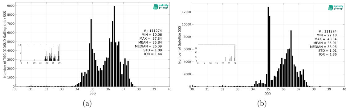
Figure 3: Histograms of SSS from TSG (GOSUD-Sailing-ship) (a) and SMOS SSS L4 OI v346 - Weekly (CMEMS-CATDS-LOPS) (b) considering all match-up pairs per bins of 0.1 over the Tropical Atlantic Ocean Pi-MEP region and for the full satellite product period.
