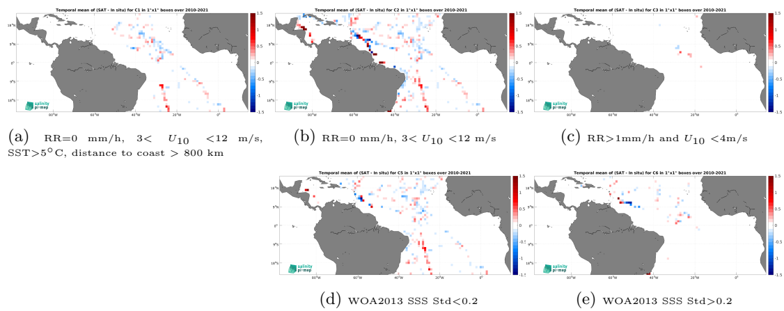
Figure 14: Temporal mean gridded over spatial boxes of size 1^\circ \times 1^\circ of \Delta\text{SSS} (SMOS SSS L4 OI v346 - Weekly (CMEMS-CATDS-LOPS) - TSG (GOSUD-Sailing-ship)) for 5 different sub-datasets corresponding to:RR=0 mm/h, 3 < U_{10} < 12 m/s, SST >5^\circ\text{C} , distance to coast > 800 km (a), RR=0 mm/h, 3 < U_{10} < 12 m/s (b), RR >1 mm/h and U_{10} < 4 m/s (c), WOA2013 SSS Std <0.2 (d), WOA2013 SSS Std >0.2 (e).
