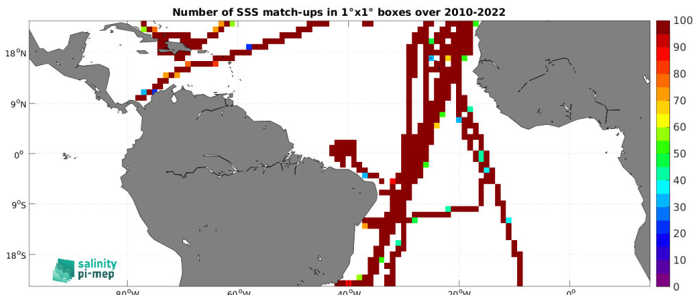
Figure 5: Number of SSS match-ups between TSG (CSIC-UTM) SSS and the SMOS SSS L4 OI v346 - Weekly (CMEMS-CATDS-LOPS) SSS product for the Tropical Atlantic Ocean Pi-MEP region over 1^\circ \times 1^\circ boxes and for the full satellite product period.
