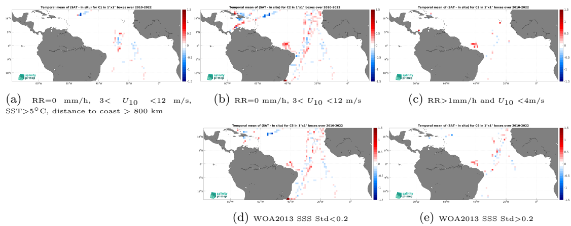
Figure 14: Temporal mean gridded over spatial boxes of size 1^\circ \times 1^\circ of \Delta\text{SSS} (SMOS SSS L4 OI v346 - Weekly (CMEMS-CATDS-LOPS) - TSG (CSIC-UTM)) for 5 different subdatasets corresponding to:RR=0 mm/h, 3 < U_{10} < 12 m/s, SST>5°C, distance to coast > 800 km (a), RR=0 mm/h, 3 < U_{10} < 12 m/s (b), RR>1mm/h and U_{10} < 4 m/s (c), WOA2013 SSS Std<0.2 (d), WOA2013 SSS Std>0.2 (e).
