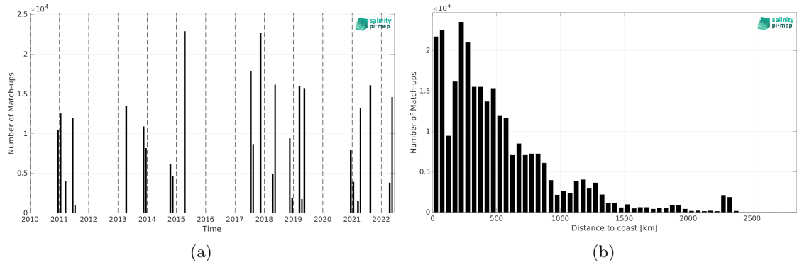
Figure 2: Number of match-ups between TSG (CSIC-UTM) and SMOS SSS L4 OI v346 - Weekly (CMEMS-CATDS-LOPS) SSS as a function of time (a) and as function of the distance to coast (b) over the Tropical Atlantic Ocean Pi-MEP region and for the full satellite product period.
