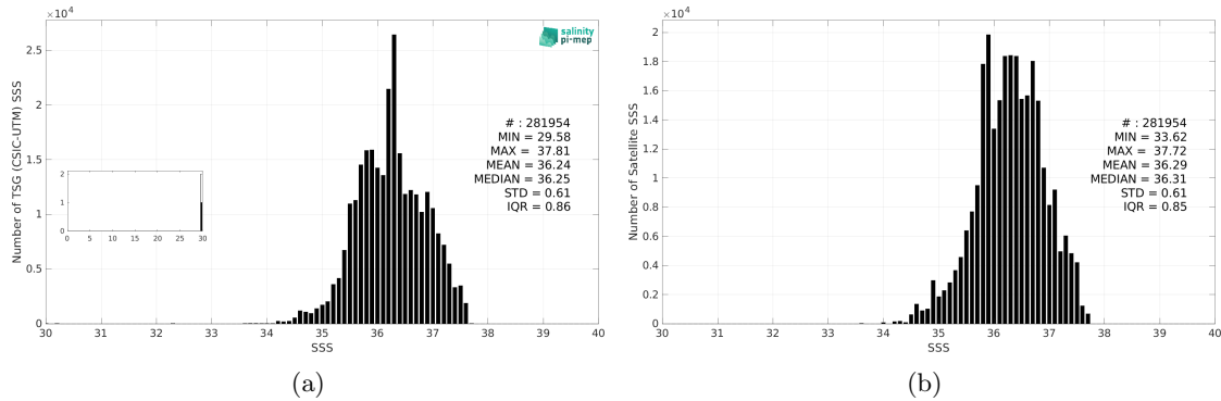
Figure 3: Histograms of SSS from TSG (CSIC-UTM) (a) and SMOS SSS L4 OI v346 - Weekly (CMEMS-CATDS-LOPS) (b) considering all match-up pairs per bins of 0.1 over the Tropical Atlantic Ocean Pi-MEP region and for the full satellite product period.
