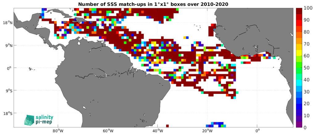
Figure 4: Number of SSS match-ups between Surface drifters SSS and the SMOS SSS L4 OI v346 - Weekly (CMEMS-CATDS-LOPS) SSS product for the Tropical Atlantic Ocean Pi-MEP region over 1^\circ \times 1^\circ boxes and for the full satellite product period.
