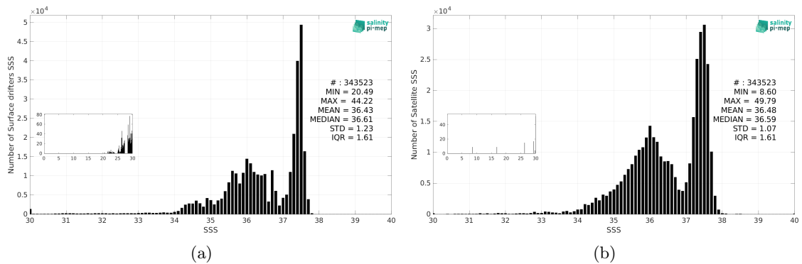
Figure 3: Histograms of SSS from Surface drifters (a) and SMOS SSS L4 OI v346 - Weekly (CMEMS-CATDS-LOPS) (b) considering all match-up pairs per bins of 0.1 over the Tropical Atlantic Ocean Pi-MEP region and for the full satellite product period.
