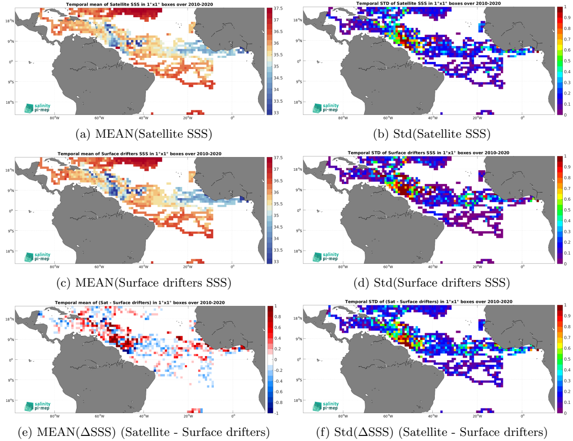
Figure 6: Temporal mean (left) and Std (right) of SSS from SMOS SSS L4 OI v346 - Weekly (CMEMS-CATDS-LOPS) (top), Surface drifters (middle), and of \Delta SSS (Satellite - Surface drifters). Only match-up pairs are used to generate these maps.
