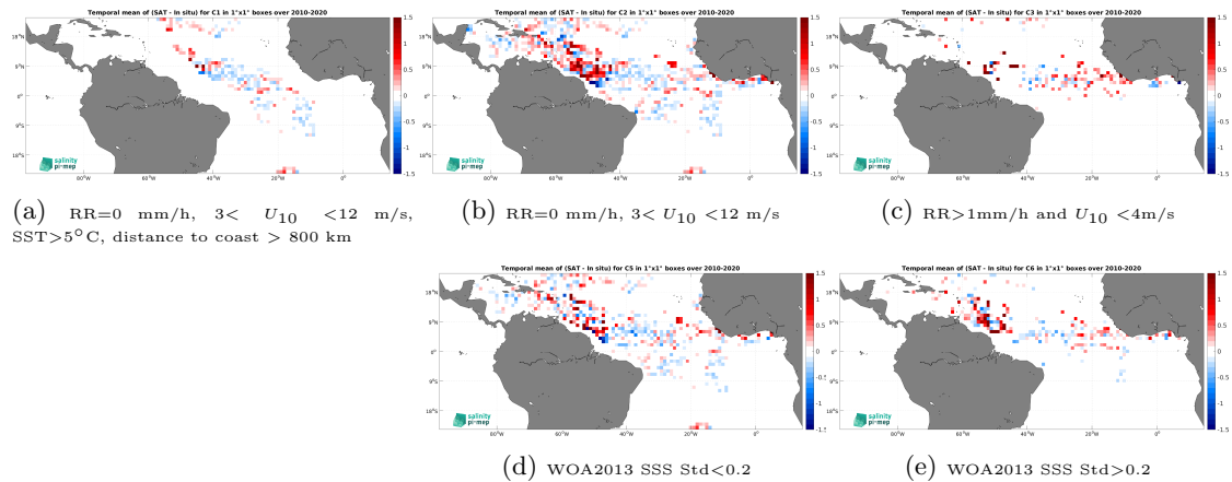
Figure 13: Temporal mean gridded over spatial boxes of size 1^\circ \times 1^\circ of \Delta\text{SSS} (SMOS SSS L4 OI v346 - Weekly (CMEMS-CATDS-LOPS) - Surface drifters) for 5 different subdatasets corresponding to:RR=0 mm/h, 3 < U_{10} < 12 m/s, SST >5^\circ\text{C} , distance to coast > 800 km (a), RR=0 mm/h, 3 < U_{10} < 12 m/s (b), RR >1 mm/h and U_{10} < 4 m/s (c), WOA2013 SSS Std <0.2 (d), WOA2013 SSS Std >0.2 (e).
