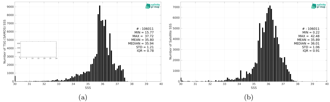
Figure 2: Histograms of SSS from TSG (SAMOS) (a) and SMOS SSS L4 OI v342 - Weekly (CMEMS-CATDS-LOPS) (b) considering all match-up pairs per bins of 0.1 over the Tropical Atlantic Ocean Pi-MEP region and for the full satellite product period.
