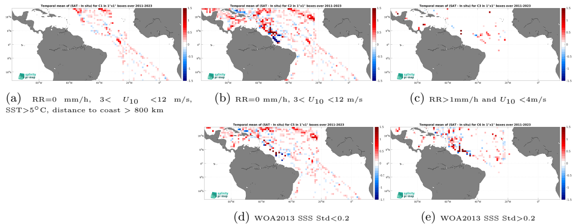
Figure 12: Temporal mean gridded over spatial boxes of size 1^\circ \times 1^\circ of \Delta\text{SSS} (SMOS SSS L4 OI v342 - Weekly (CMEMS-CATDS-LOPS) - TSG (SAMOS)) for 5 different subdatasets corresponding to:RR=0 mm/h, 3 < U_{10} < 12 m/s, SST >5^\circ\text{C} , distance to coast > 800 km (a), RR=0 mm/h, 3 < U_{10} < 12 m/s (b), RR >1 mm/h and U_{10} < 4 m/s (c), WOA2013 SSS Std <0.2 (d), WOA2013 SSS Std >0.2 (e).
