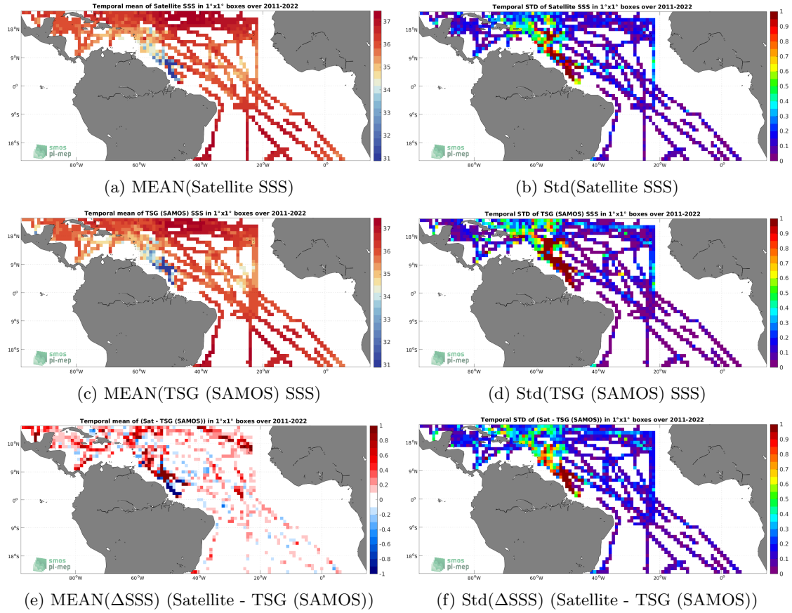
Figure 6: Temporal mean (left) and Std (right) of SSS from SMOS SSS L4 OI v342 - Weekly (CMEMS-CATDS-LOPS) (top), TSG (SAMOS) (middle), and of \Delta SSS (Satellite - TSG (SAMOS)). Only match-up pairs are used to generate these maps.
