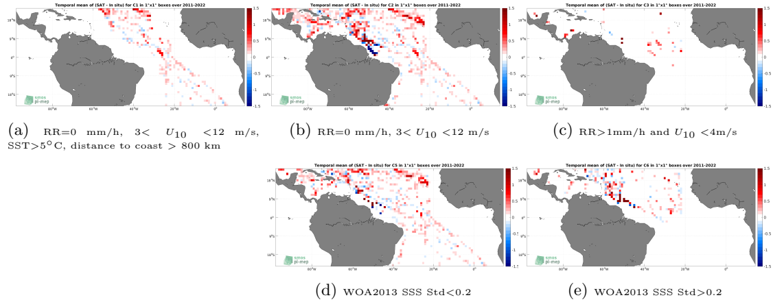
Figure 12: Temporal mean gridded over spatial boxes of size 1^{\circ}\times 1^{\circ} of \Delta\text{SSS} (SMOS SSS L4 OI v342 - Weekly (CMEMS-CATDS-LOPS) - TSG (SAMOS)) for 5 different subdatasets corresponding to: RR=0 mm/h, 3 < U_{10} < 12 m/s, SST > 5^{\circ}\text{C} , distance to coast > 800 km (a), RR=0 mm/h, 3 < U_{10} < 12 m/s (b), RR > 1 mm/h and U_{10} < 4 m/s (c), WOA2013 SSS Std < 0.2 (d), WOA2013 SSS Std > 0.2 (e).
