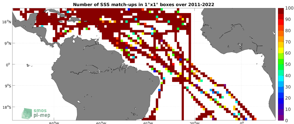
Figure 4: Number of SSS match-ups between TSG (SAMOS) SSS and the SMOS SSS L4 OI v342 - Weekly (CMEMS-CATDS-LOPS) SSS product for the Tropical Atlantic Ocean Pi-MEP region over 1^\circ \times 1^\circ boxes and for the full satellite product period.
