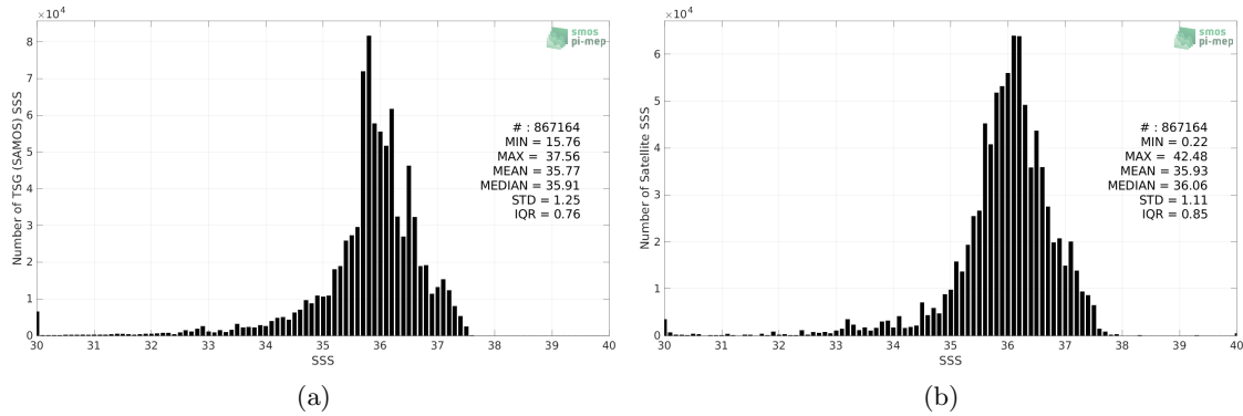
Figure 2: Histograms of SSS from TSG (SAMOS) (a) and SMOS SSS L4 OI v342 - Weekly (CMEMS-CATDS-LOPS) (b) considering all match-up pairs per bins of 0.1 over the Tropical Atlantic Ocean Pi-MEP region and for the full satellite product period.
