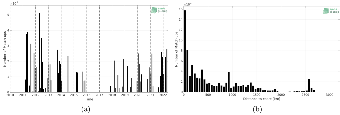
Figure 1: Number of match-ups between TSG (SAMOS) and SMOS SSS L4 OI v342 - Weekly (CMEMS-CATDS-LOPS) SSS as a function of time (a) and as function of the distance to coast (b) over the Tropical Atlantic Ocean Pi-MEP region and for the full satellite product period.
