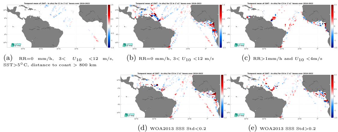
Figure 12: Temporal mean gridded over spatial boxes of size 1^\circ \times 1^\circ of \Delta\text{SSS} (SMOS SSS L4 OI v342 - Weekly (CMEMS-CATDS-LOPS) - TSG (LEGOS-DM)) for 5 different subdatasets corresponding to:RR=0 mm/h, 3 < U_{10} < 12 m/s, SST >5^\circ\text{C} , distance to coast > 800 km (a), RR=0 mm/h, 3 < U_{10} < 12 m/s (b), RR >1 mm/h and U_{10} < 4 m/s (c), WOA2013 SSS Std <0.2 (d), WOA2013 SSS Std >0.2 (e).
