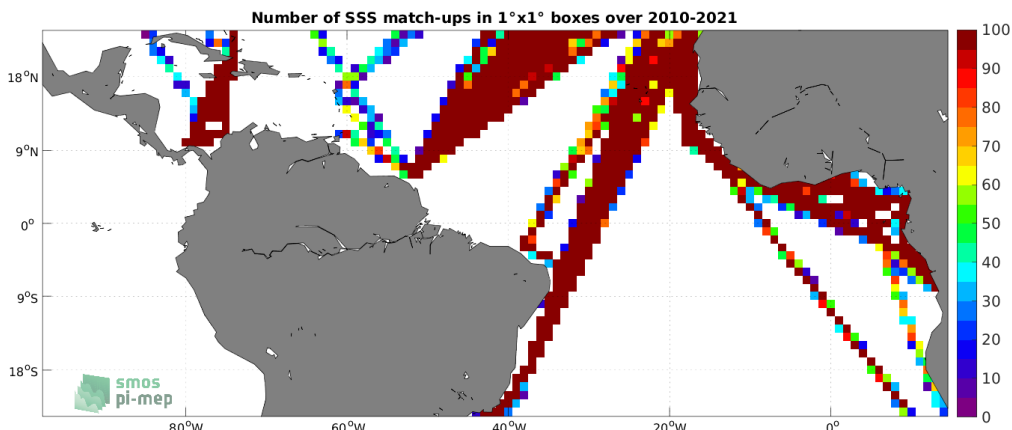
Figure 4: Number of SSS match-ups between TSG (LEGOS-DM) SSS and the SMOS SSS L4 OI v342 - Weekly (CMEMS-CATDS-LOPS) SSS product for the Tropical Atlantic Ocean Pi-MEP region over 1^\circ \times 1^\circ boxes and for the full satellite product period.
