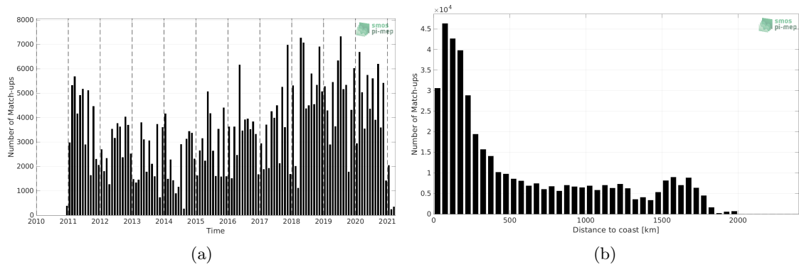
Figure 1: Number of match-ups between TSG (LEGOS-DM) and SMOS SSS L4 OI v342 - Weekly (CMEMS-CATDS-LOPS) SSS as a function of time (a) and as function of the distance to coast (b) over the Tropical Atlantic Ocean Pi-MEP region and for the full satellite product period.
