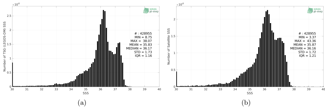
Figure 2: Histograms of SSS from TSG (LEGOS-DM) (a) and SMOS SSS L4 OI v342 - Weekly (CMEMS-CATDS-LOPS) (b) considering all match-up pairs per bins of 0.1 over the Tropical Atlantic Ocean Pi-MEP region and for the full satellite product period.
