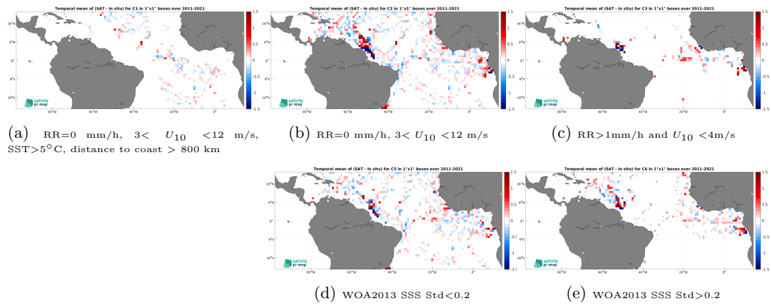
Figure 12: Temporal mean gridded over spatial boxes of size 1^\circ \times 1^\circ of \Delta SSS (SMOS SSS L4 OI v342 - Weekly (CMEMS-CATDS-LOPS) - TSG (GOSUD-Research-vessel)) for 5 different subdatasets corresponding to:RR=0 mm/h, 3 < U_{10} < 12 m/s, SST >5^\circ\text{C} , distance to coast > 800 km (a), RR=0 mm/h, 3 < U_{10} < 12 m/s (b), RR >1 mm/h and U_{10} < 4 m/s (c), WOA2013 SSS Std <0.2 (d), WOA2013 SSS Std >0.2 (e).
