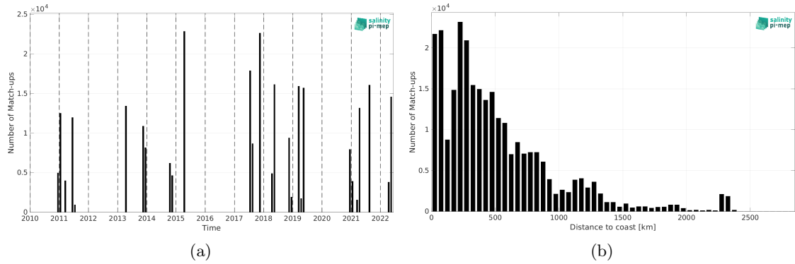
Figure 1: Number of match-ups between TSG (CSIC-UTM) and SMOS SSS L4 OI v342 - Weekly (CMEMS-CATDS-LOPS) SSS as a function of time (a) and as function of the distance to coast (b) over the Tropical Atlantic Ocean Pi-MEP region and for the full satellite product period.
