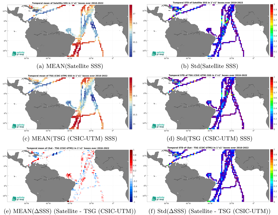
Figure 6: Temporal mean (left) and Std (right) of SSS from SMOS SSS L4 OI v342 - Weekly (CMEMS-CATDS-LOPS) (top), TSG (CSIC-UTM) (middle), and of \Delta SSS (Satellite - TSG (CSIC-UTM)). Only match-up pairs are used to generate these maps.
