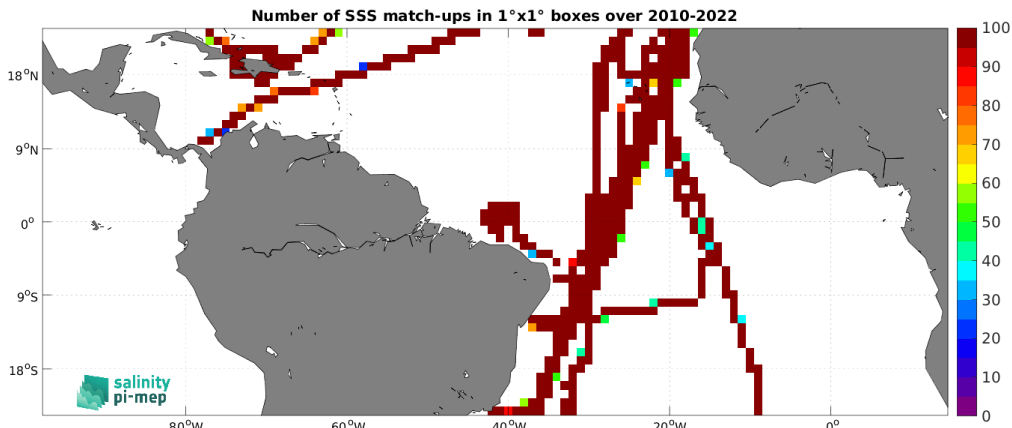
Figure 4: Number of SSS match-ups between TSG (CSIC-UTM) SSS and the SMOS SSS L4 OI v342 - Weekly (CMEMS-CATDS-LOPS) SSS product for the Tropical Atlantic Ocean Pi-MEP region over 1^\circ \times 1^\circ boxes and for the full satellite product period.
