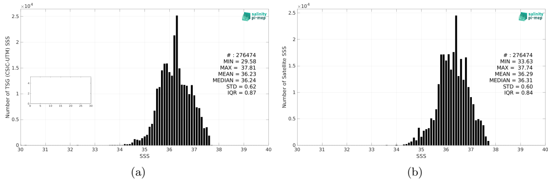
Figure 2: Histograms of SSS from TSG (CSIC-UTM) (a) and SMOS SSS L4 OI v342 - Weekly (CMEMS-CATDS-LOPS) (b) considering all match-up pairs per bins of 0.1 over the Tropical Atlantic Ocean Pi-MEP region and for the full satellite product period.
