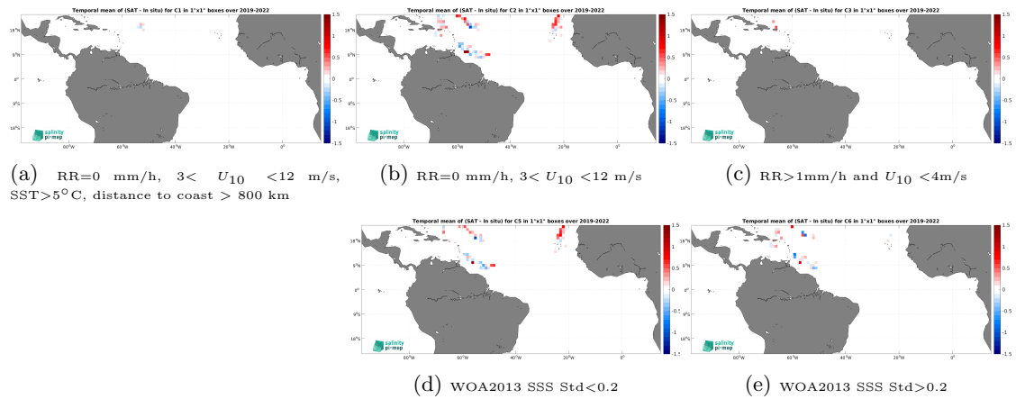
Figure 12: Temporal mean gridded over spatial boxes of size 1^\circ \times 1^\circ of \Delta\text{SSS} (SMOS SSS L4 OI v342 - Weekly (CMEMS-CATDS-LOPS) - Sailydrone) for 5 different subdatasets corresponding to:RR=0 mm/h, 3 < U_{10} < 12 m/s, SST >5^\circ\text{C} , distance to coast > 800 km (a), RR=0 mm/h, 3 < U_{10} < 12 m/s (b), RR >1 mm/h and U_{10} < 4 m/s (c), WOA2013 SSS Std <0.2 (d), WOA2013 SSS Std >0.2 (e).
