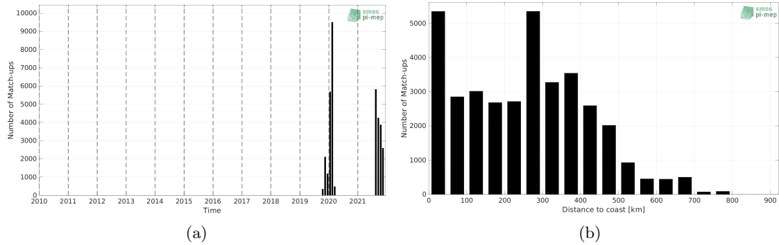
Figure 1: Number of match-ups between Saildrone and SMOS SSS L4 OI v342 - Weekly (CMEMS-CATDS-LOPS) SSS as a function of time (a) and as function of the distance to coast (b) over the Tropical Atlantic Ocean Pi-MEP region and for the full satellite product period.
