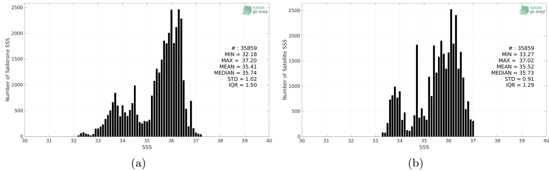
Figure 2: Histograms of SSS from Saildrone (a) and SMOS SSS L4 OI v342 - Weekly (CMEMS-CATDS-LOPS) (b) considering all match-up pairs per bins of 0.1 over the Tropical Atlantic Ocean Pi-MEP region and for the full satellite product period.
