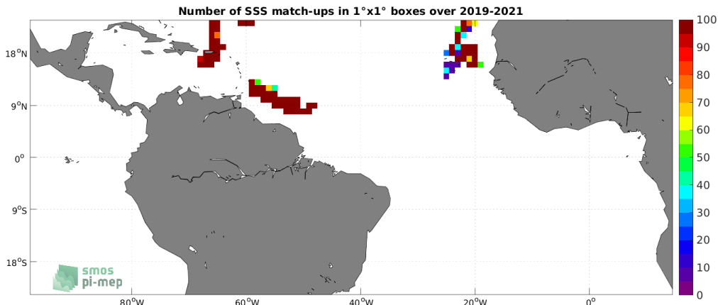
Figure 4: Number of SSS match-ups between Saildrone SSS and the SMOS SSS L4 OI v342 - Weekly (CMEMS-CATDS-LOPS) SSS product for the Tropical Atlantic Ocean Pi-MEP region over 1^\circ \times 1^\circ boxes and for the full satellite product period.
