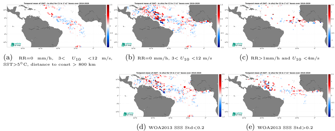
Figure 11: Temporal mean gridded over spatial boxes of size 1^\circ \times 1^\circ of \Delta SSS (SMOS SSS L4 OI v342 - Weekly (CMEMS-CATDS-LOPS) - Surface drifters) for 5 different subdatasets corresponding to:RR=0 mm/h, 3 < U_{10} < 12 m/s, SST >5^\circ C, distance to coast > 800 km (a), RR=0 mm/h, 3 < U_{10} < 12 m/s (b), RR >1 mm/h and U_{10} < 4 m/s (c), WOA2013 SSS Std <0.2 (d), WOA2013 SSS Std >0.2 (e).
