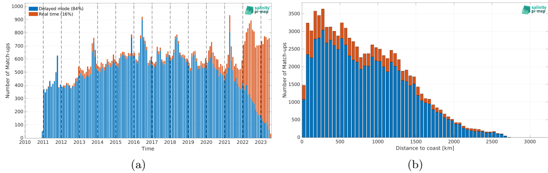
Figure 1: Number of match-ups between Argo and SMOS SSS L4 OI v342 - Weekly (CMEMS-CATDS-LOPS) SSS as a function of time (a) and as function of the distance to coast (b) over the Tropical Atlantic Ocean Pi-MEP region and for the full satellite product period.
