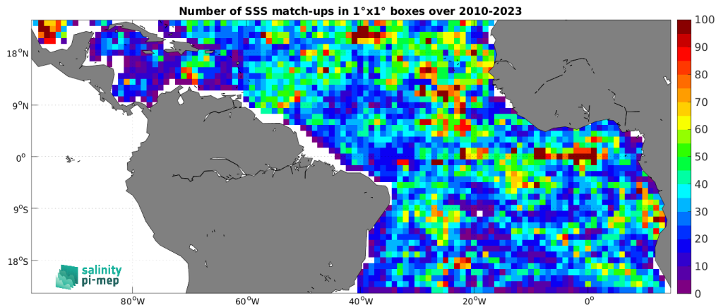
Figure 4: Number of SSS match-ups between Argo SSS and the SMOS SSS L4 OI v342 - Weekly (CMEMS-CATDS-LOPS) SSS product for the Tropical Atlantic Ocean Pi-MEP region over 1^\circ \times 1^\circ boxes and for the full satellite product period.
