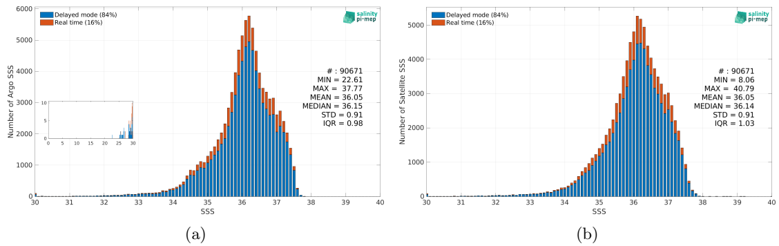
Figure 2: Histograms of SSS from Argo (a) and SMOS SSS L4 OI v342 - Weekly (CMEMS-CATDS-LOPS) (b) considering all match-up pairs per bins of 0.1 over the Tropical Atlantic Ocean Pi-MEP region and for the full satellite product period.
