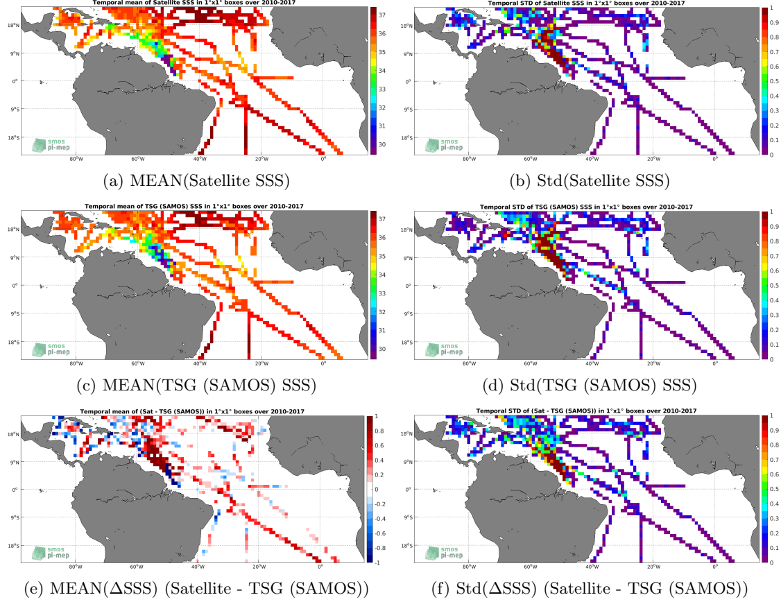
Figure 6: Temporal mean (left) and Std (right) of SSS from SMOS L4 v2 Weekly (CATDS-CECOS-IFREMER) (top), TSG (SAMOS) (middle), and of \Delta\text{SSS} (Satellite - TSG (SAMOS)). Only match-up pairs are used to generate these maps.
