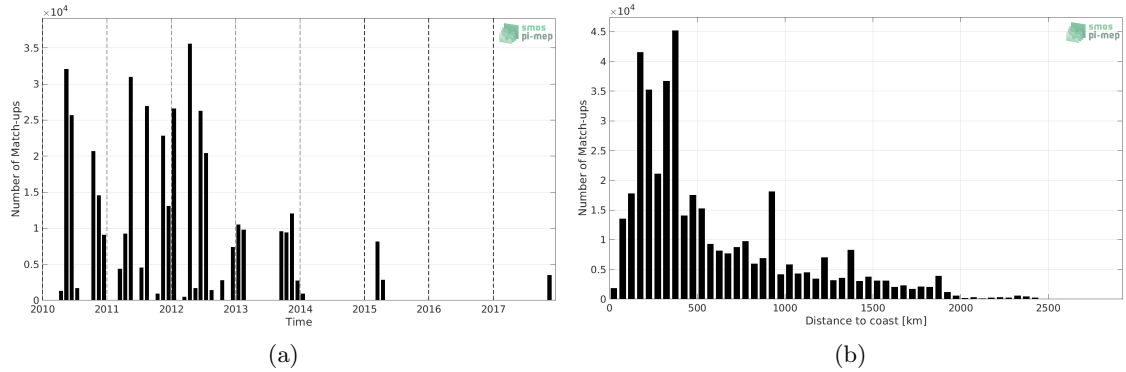
Figure 1: Number of match-ups between TSG (SAMOS) and SMOS L4 v2 Weekly (CATDS-CECOS-IFREMER) SSS as a function of TSG (a) and as function of the distance to coast (b) over the Tropical Atlantic Ocean Pi-MEP region and for the full satellite product period.
