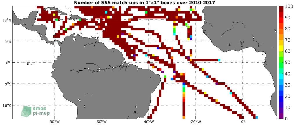
Figure 4: Number of SSS match-ups between TSG (SAMOS) SSS and the SMOS L4 v2 Weekly (CATDS-CECOS-IFREMER) SSS product for the Tropical Atlantic Ocean Pi-MEP region over 1^\circ \times 1^\circ boxes and for the full satellite product period.
