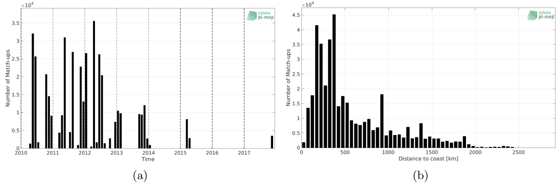
Figure 1: Number of match-ups between TSG (SAMOS) and SMOS L4 v2 Weekly (CATDS-CECOS-IFREMER) SSS as a function of time (a) and as function of the distance to coast (b) over the Tropical Atlantic Ocean Pi-MEP region and for the full satellite product period.
