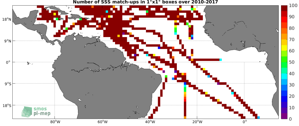
Figure 4: Number of SSS match-ups between TSG (SAMOS) SSS and the SMOS L4 v2 Weekly (CATDS-CECOS-IFREMER) SSS product for the Tropical Atlantic Ocean Pi-MEP region over 1°x1° boxes and for the full satellite product period.
