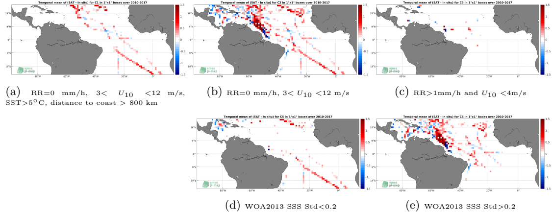
Figure 12: Temporal mean gridded over spatial boxes of size 1^{\circ}\times 1^{\circ} of \Delta\text{SSS} (SMOS L4 v2 Weekly (CATDS-CECOS-IFREMER) - TSG (SAMOS)) for 5 different subdatasets corresponding to:RR=0 mm/h, 3 < U_{10} < 12 m/s, SST >5^{\circ}\text{C} , distance to coast > 800 km (a), RR=0 mm/h, 3 < U_{10} < 12 m/s (b), RR >1 mm/h and U_{10} < 4 m/s (c), WOA2013 SSS Std <0.2 (d), WOA2013 SSS Std >0.2 (e).
