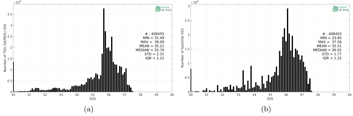
Figure 2: Histograms of SSS from TSG (SAMOS) (a) and SMOS L4 v2 Weekly (CATDS-CECOS-IFREMER) (b) considering all match-up pairs per bins of 0.1 over the Tropical Atlantic Ocean Pi-MEP region and for the full satellite product period.
