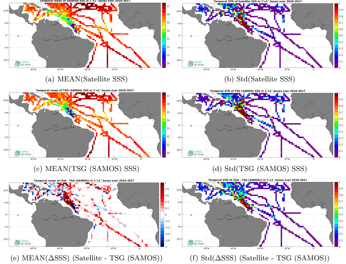
Figure 6: Temporal mean (left) and Std (right) of SSS from SMOS L4 v2 Weekly (CATDS-CECOS-IFREMER) (top), TSG (SAMOS) (middle), and of \Delta SSS (Satellite - TSG (SAMOS)). Only match-up pairs are used to generate these maps.
