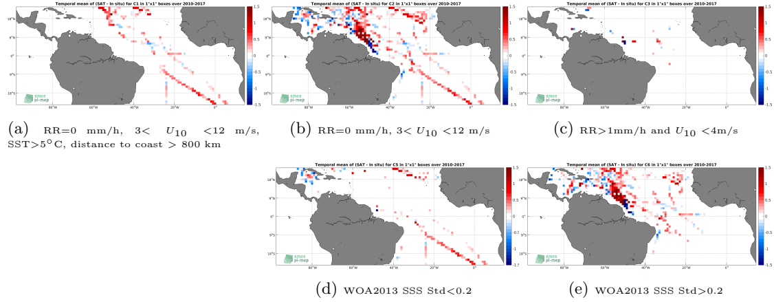
Figure 12: Temporal mean gridded over spatial boxes of size 1^{\circ}\times 1^{\circ} of \Delta\text{SSS} (SMOS-L4-CATDS-CECOS-IFREMER-V2-WEEKLY-0.5DEG - TSG-SAMOS) for 5 different subdatasets corresponding to: \text{RR}=0 mm/h, 3 < U_{10} < 12 m/s, \text{SST} > 5^{\circ}\text{C} , distance to coast > 800 km (a), \text{RR}=0 mm/h, 3 < U_{10} < 12 m/s (b), \text{RR} > 1 mm/h and U_{10} < 4 m/s (c), WOA2013 SSS Std < 0.2 (d), WOA2013 SSS Std > 0.2 (e).
