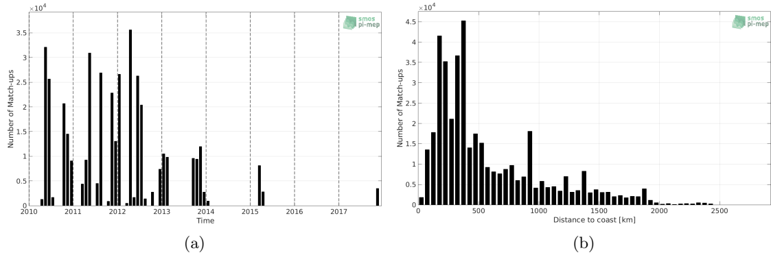
Figure 1: Number of match-ups between TSG-SAMOS and SMOS-L4-CATDS-CECOS-IFREMER-V2-WEEKLY-0.5DEG SSS as a function of time (a) and as function of the distance to coast (b) over the Tropical Atlantic Ocean Pi-MEP region and for the full satellite product period.
