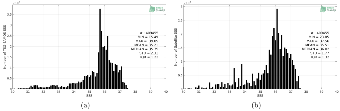
Figure 2: Histograms of SSS from TSG-SAMOS (a) and SMOS-L4-CATDS-CECOS-IFREMER-V2-WEEKLY-0.5DEG (b) considering all match-up pairs per bins of 0.1 over the Tropical Atlantic Ocean Pi-MEP region and for the full satellite product period.
