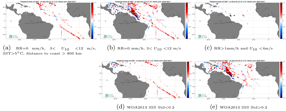
Figure 12: Temporal mean gridded over spatial boxes of size 1^\circ \times 1^\circ of \Delta SSS (SMOS-L4-CATDS-CECOS-IFREMER-V2-WEEKLY-0.5DEG - TSG-SAMOS) for 5 different subdatasets corresponding to: RR=0 mm/h, 3 < U_{10} < 12 m/s, SST > 5^\circ C , distance to coast > 800 km (a), RR=0 mm/h, 3 < U_{10} < 12 m/s (b), RR > 1 mm/h and U_{10} < 4 m/s (c), WOA2013 SSS Std < 0.2 (d), WOA2013 SSS Std > 0.2 (e).
