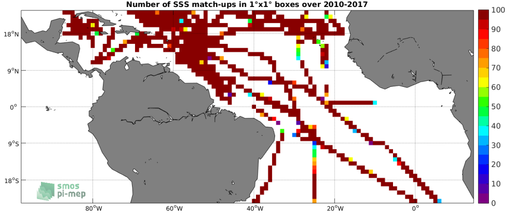
Figure 4: Number of SSS match-ups between TSG-SAMOS SSS and the SMOS-L4-CATDS-CECOS-IFREMER-V2-WEEKLY-0.5DEG SSS product for the Tropical Atlantic Ocean Pi-MEP region over 1°x1° boxes and for the full satellite product period.
