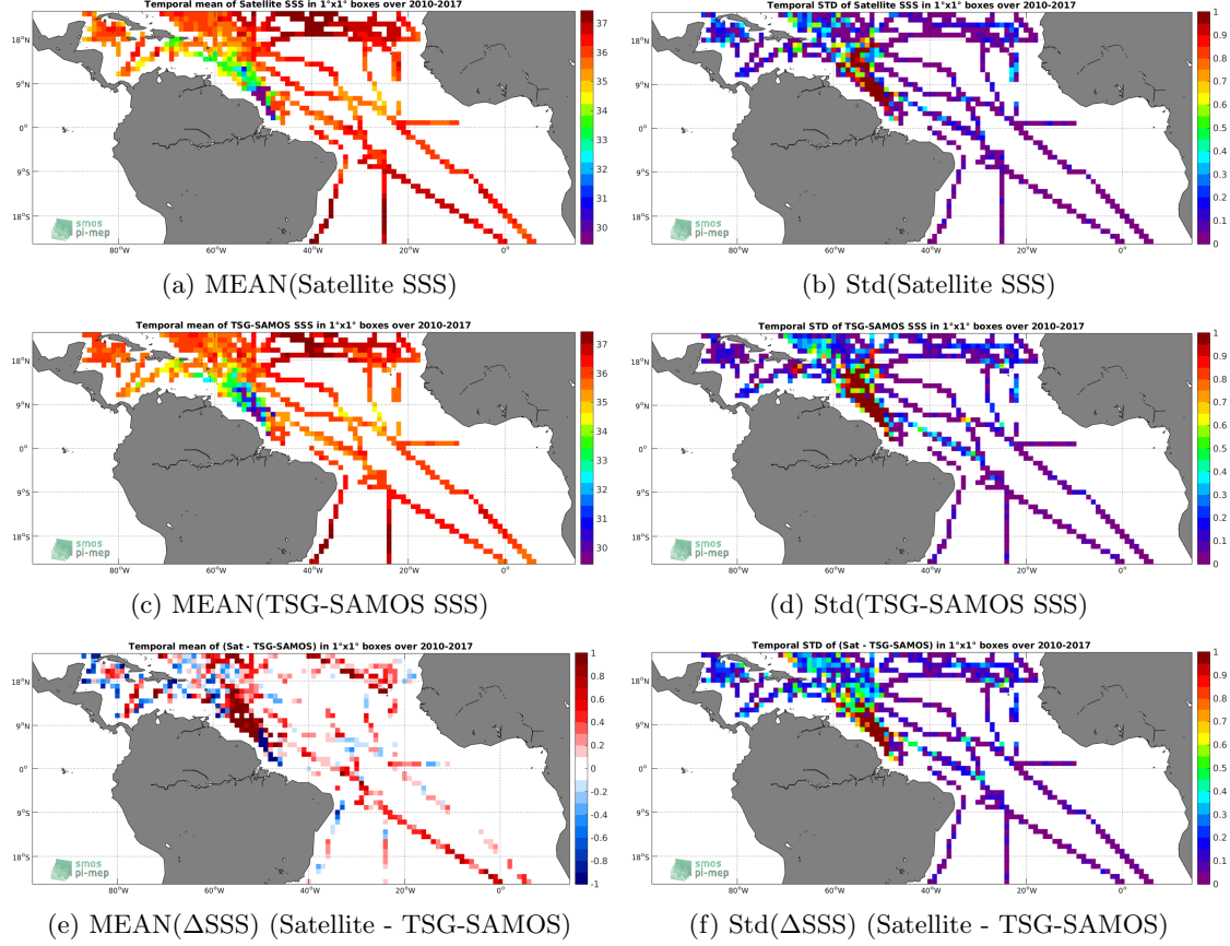
Figure 6: Temporal mean (left) and Std (right) of SSS from SMOS-L4-CATDS-CECOS-IFREMER-V2-WEEKLY-0.5DEG (top), TSG-SAMOS (middle), and of \Delta SSS (Satellite - TSG-SAMOS). Only match-up pairs are used to generate these maps.
