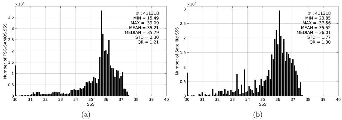
Figure 2: Histograms of SSS from TSG-SAMOS (a) and SMOS-L4-CATDS-CECOS-IFREMER-V2-WEEKLY-0.5DEG (b) considering all match-up pairs per bins of 0.1 over the Tropical Atlantic Ocean Pi-MEP region and for the full satellite product period.
