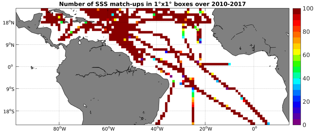
Figure 4: Number of SSS match-ups between TSG-SAMOS SSS and the SMOS-L4-CATDS-CECOS-IFREMER-V2-WEEKLY-0.5DEG SSS product for the Tropical Atlantic Ocean Pi-MEP region over 1°x1° boxes and for the full satellite product period.
