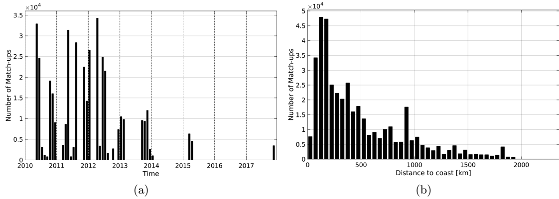
Figure 1: Number of match-ups between TSG-SAMOS and SMOS-L4-CATDS-CECOS-IFREMER-V2-WEEKLY-0.5DEG SSS as a function of time (a) and as function of the distance to coast (b) over the Tropical Atlantic Ocean Pi-MEP region and for the full satellite product period.
