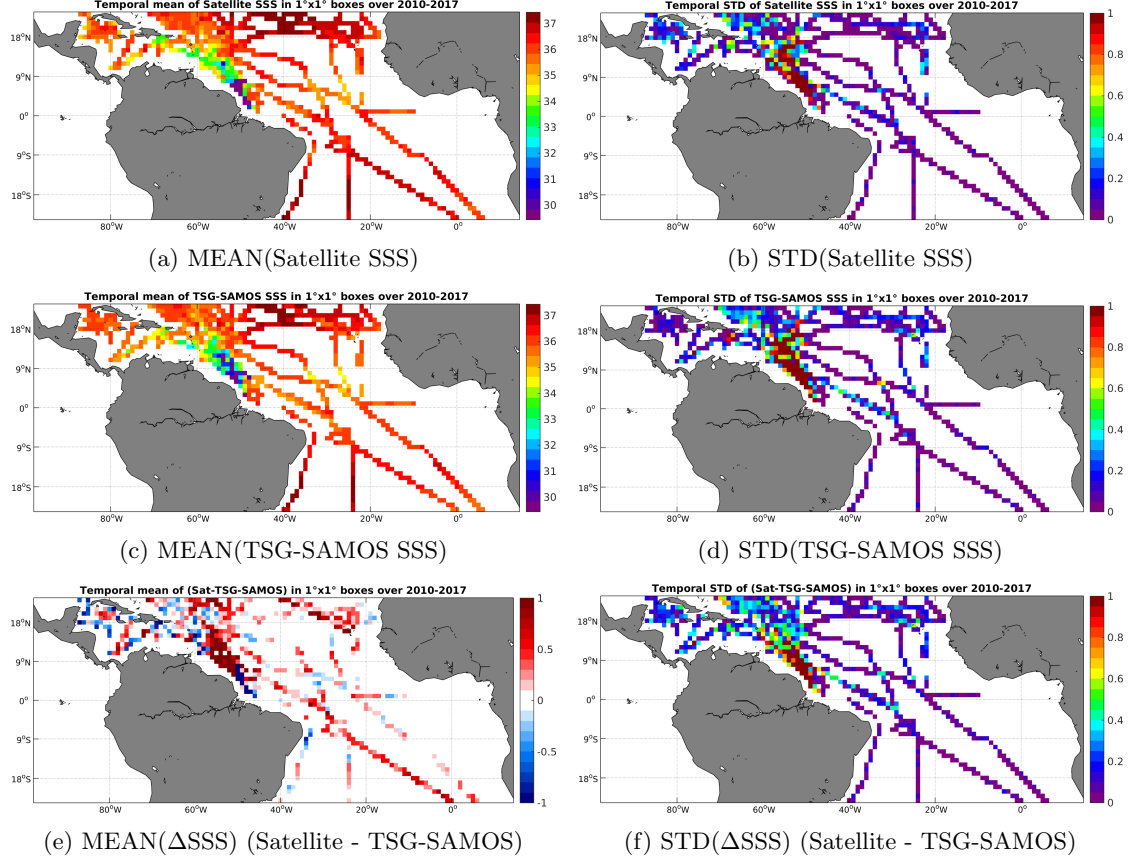
Figure 6: Temporal mean (left) and STD (right) of SSS from SMOS-L4-CATDS-CECOS-IFREMER-V2-WEEKLY-0.5DEG (top), TSG-SAMOS (middle), and of \Delta\text{SSS} (Satellite - TSG-SAMOS). Only match-up pairs are used to generate these maps.
