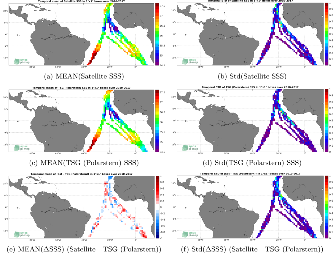
Figure 6: Temporal mean (left) and Std (right) of SSS from SMOS L4 v2 Weekly (CATDS-CECOS-IFREMER) (top), TSG (Polarstern) (middle), and of \Delta\text{SSS} (Satellite - TSG (Polarstern)). Only match-up pairs are used to generate these maps.
