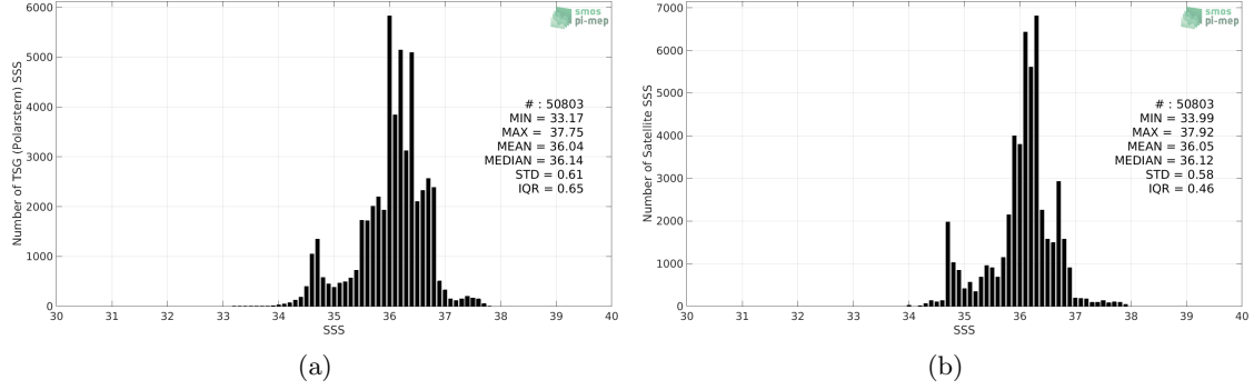
Figure 2: Histograms of SSS from TSG (Polarstern) (a) and SMOS L4 v2 Weekly (CATDS-CECOS-IFREMER) (b) considering all match-up pairs per bins of 0.1 over the Tropical Atlantic Ocean Pi-MEP region and for the full satellite product period.
