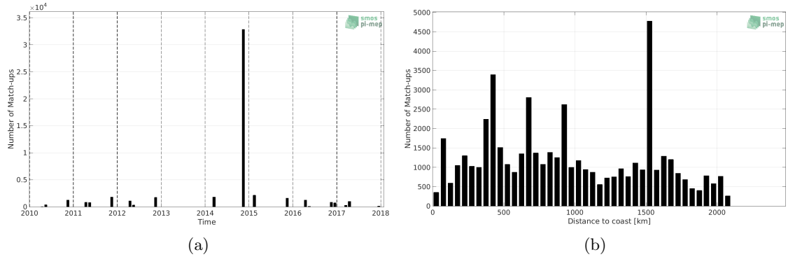
Figure 1: Number of match-ups between TSG (Polarstern) and SMOS L4 v2 Weekly (CATDS-CECOS-IFREMER) SSS as a function of time (a) and as function of the distance to coast (b) over the Tropical Atlantic Ocean Pi-MEP region and for the full satellite product period.
