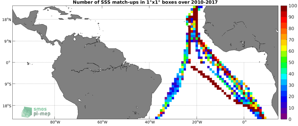
Figure 4: Number of SSS match-ups between TSG (Polarstern) SSS and the SMOS L4 v2 Weekly (CATDS-CECOS-IFREMER) SSS product for the Tropical Atlantic Ocean Pi-MEP region over 1^\circ \times 1^\circ boxes and for the full satellite product period.
