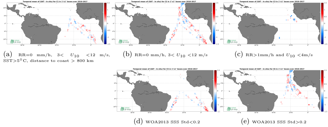
Figure 12: Temporal mean gridded over spatial boxes of size 1^{\circ}\times 1^{\circ} of \Delta\text{SSS} (SMOS L4 v2 Weekly (CATDS-CECOS-IFREMER) - TSG (Polarstern)) for 5 different subdatasets corresponding to: \text{RR}=0 mm/h, 3 < U_{10} < 12 m/s, \text{SST}>5^{\circ}\text{C} , distance to coast > 800 km (a), \text{RR}=0 mm/h, 3 < U_{10} < 12 m/s (b), \text{RR}>1\text{mm/h} and U_{10} < 4\text{m/s} (c), WOA2013 SSS Std <0.2 (d), WOA2013 SSS Std >0.2 (e).
