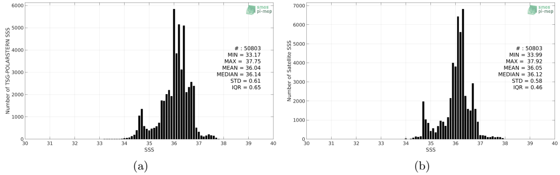
Figure 2: Histograms of SSS from TSG-POLARSTERN (a) and SMOS-L4-CATDS-CECOS-IFREMER-V2-WEEKLY-0.5DEG (b) considering all match-up pairs per bins of 0.1 over the Tropical Atlantic Ocean Pi-MEP region and for the full satellite product period.
