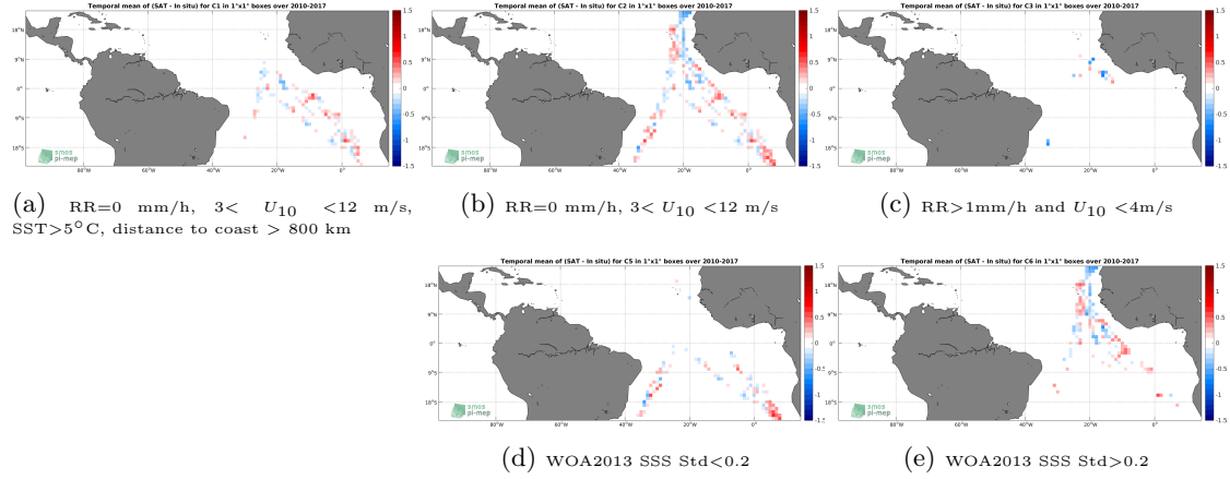
Figure 12: Temporal mean gridded over spatial boxes of size 1^{\circ}\times 1^{\circ} of \Delta\text{SSS} (SMOS-L4-CATDS-CECOS-IFREMER-V2-WEEKLY-0.5DEG - TSG-POLARSTERN) for 5 different subdatasets corresponding to: RR=0 mm/h, 3 < U_{10} < 12 m/s, SST > 5^{\circ}\text{C} , distance to coast > 800 km (a), RR=0 mm/h, 3 < U_{10} < 12 m/s (b), RR > 1 mm/h and U_{10} < 4 m/s (c), WOA2013 SSS Std < 0.2 (d), WOA2013 SSS Std > 0.2 (e).
