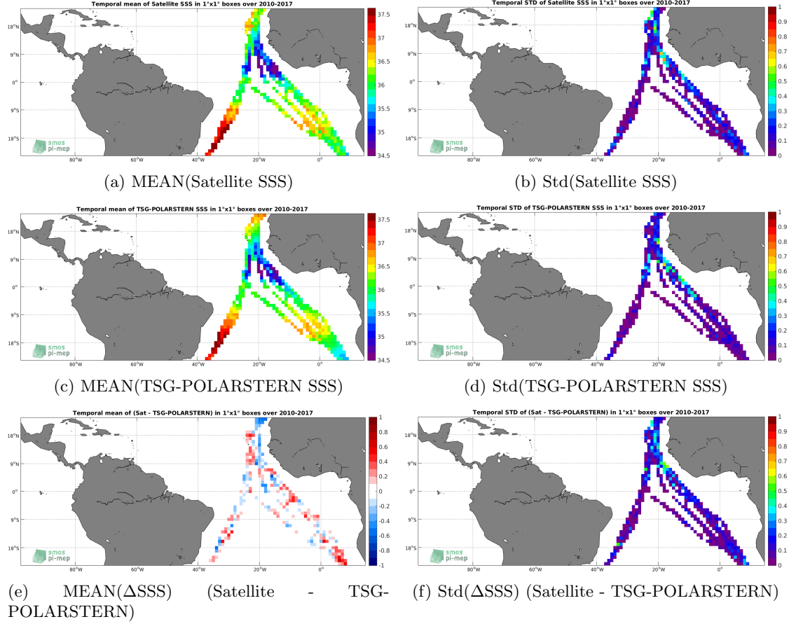
Figure 6: Temporal mean (left) and Std (right) of SSS from SMOS-L4-CATDS-CECOS-IFREMER-V2-WEEKLY-0.5DEG (top), TSG-POLARSTERN (middle), and of \Delta\text{SSS} (Satellite - TSG-POLARSTERN). Only match-up pairs are used to generate these maps.
