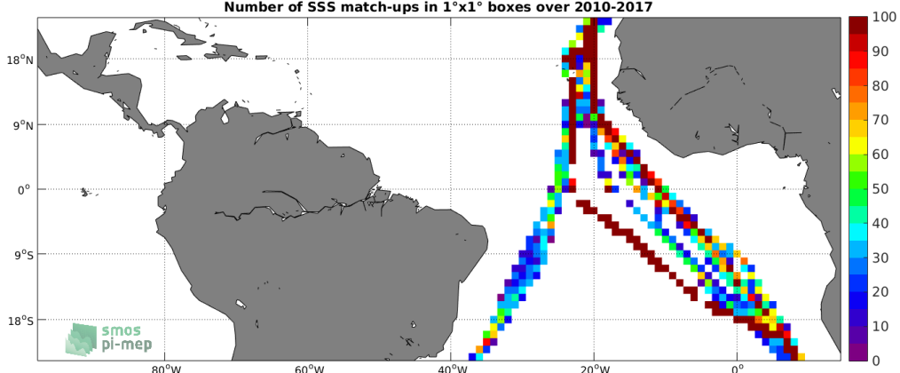
Figure 4: Number of SSS match-ups between TSG-POLARSTERN SSS and the SMOS-L4-CATDS-CECOS-IFREMER-V2-WEEKLY-0.5DEG SSS product for the Tropical Atlantic Ocean Pi-MEP region over 1^\circ \times 1^\circ boxes and for the full satellite product period.
