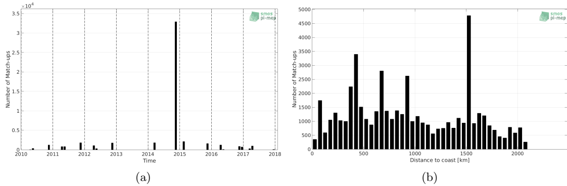
Figure 1: Number of match-ups between TSG-POLARSTERN and SMOS-L4-CATDS-CECOS-IFREMER-V2-WEEKLY-0.5DEG SSS as a function of time (a) and as function of the distance to coast (b) over the Tropical Atlantic Ocean Pi-MEP region and for the full satellite product period.
