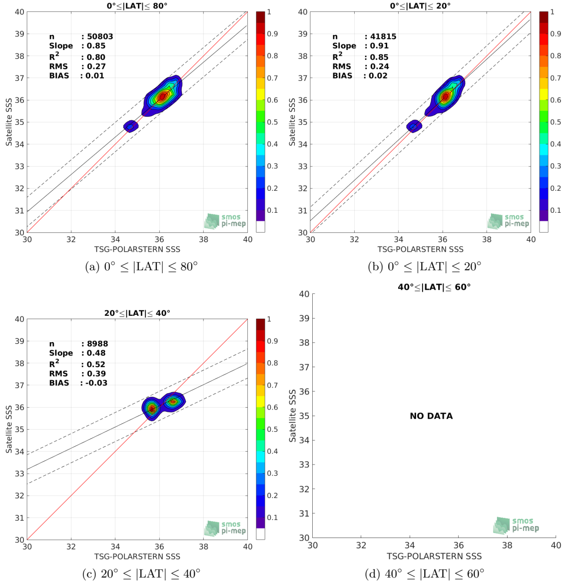
Figure 9: Contour maps of the concentration of SMOS-L4-CATDS-CECOS-IFREMER-V2-WEEKLY-0.5DEG SSS (y-axis) versus TSG-POLARSTERN SSS (x-axis) at match-up pairs for different latitude bands. For each plot, the red line shows x=y . The black thin and dashed lines indicate a linear fit through the data cloud and the \pm 95\% confidence levels, respectively. The number match-up pairs n , the slope and R^2 coefficient of the linear fit, the root mean square (RMS) and the mean bias between satellite and in situ data are indicated for each latitude band in each plots.
