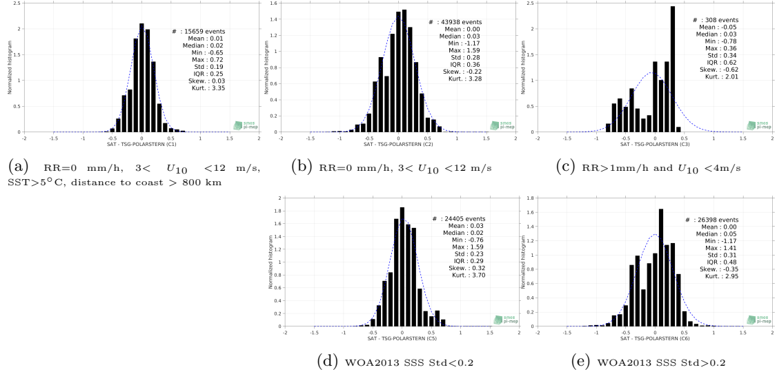
Figure 13: Normalized histogram of \Delta SSS (SMOS-L4-CATDS-CECOS-IFREMER-V2-WEEKLY-0.5DEG - TSG-POLARSTERN) for 5 different subdatasets corresponding to: RR=0 mm/h, 3 < U_{10} < 12 m/s, SST > 5°C, distance to coast > 800 km (a), RR=0 mm/h, 3 < U_{10} < 12 m/s (b), RR > 1mm/h and U_{10} < 4 m/s (c), WOA2013 SSS Std < 0.2 (d), WOA2013 SSS Std > 0.2 (e).
