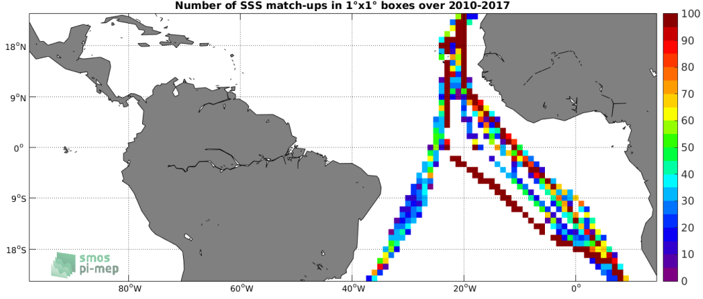
Figure 4: Number of SSS match-ups between TSG-POLARSTERN SSS and the SMOS-L4-CATDS-CECOS-IFREMER-V2-WEEKLY-0.5DEG SSS product for the Tropical Atlantic Ocean Pi-MEP region over 1^\circ \times 1^\circ boxes and for the full satellite product period.
