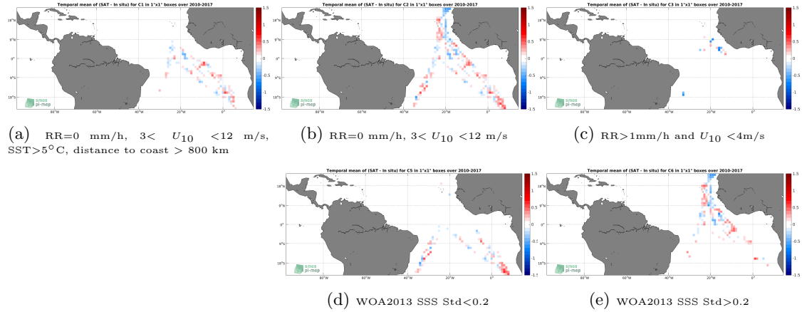
Figure 12: Temporal mean gridded over spatial boxes of size 1^\circ \times 1^\circ of \Delta SSS (SMOS-L4-CATDS-CECOS-IFREMER-V2-WEEKLY-0.5DEG - TSG-POLARSTERN) for 5 different subdatasets corresponding to: RR=0 mm/h, 3 < U_{10} < 12 m/s, SST > 5^\circ C , distance to coast > 800 km (a), RR=0 mm/h, 3 < U_{10} < 12 m/s (b), RR > 1 mm/h and U_{10} < 4 m/s (c), WOA2013 SSS Std < 0.2 (d), WOA2013 SSS Std > 0.2 (e).
