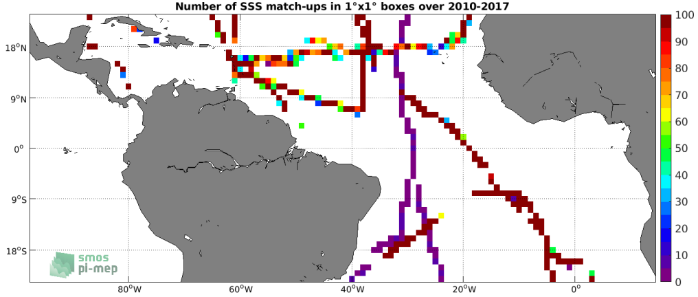
Figure 4: Number of SSS match-ups between TSG (GOSUD-Sailing-ship) SSS and the SMOS L4 v2 Weekly (CATDS-CECOS-IFREMER) SSS product for the Tropical Atlantic Ocean Pi-MEP region over 1^\circ \times 1^\circ boxes and for the full satellite product period.
