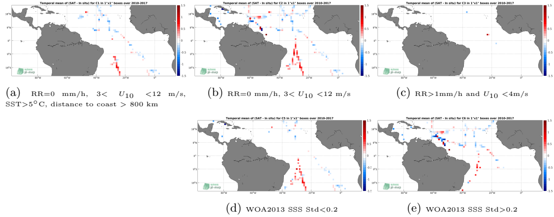
Figure 12: Temporal mean gridded over spatial boxes of size 1^{\circ}\times 1^{\circ} of \Delta SSS (SMOS L4 v2 Weekly (CATDS-CECOS-IFREMER) - TSG (GOSUD-Sailing-ship)) for 5 different subdatasets corresponding to:RR=0 mm/h, 3 < U_{10} < 12 m/s, SST >5^{\circ}\text{C} , distance to coast > 800 km (a), RR=0 mm/h, 3 < U_{10} < 12 m/s (b), RR >1 mm/h and U_{10} < 4 m/s (c), WOA2013 SSS Std <0.2 (d), WOA2013 SSS Std >0.2 (e).
