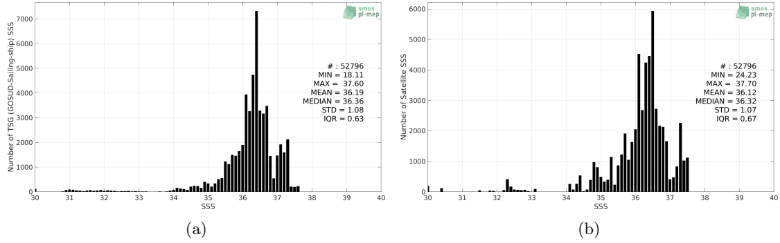
Figure 2: Histograms of SSS from TSG (GOSUD-Sailing-ship) (a) and SMOS L4 v2 Weekly (CATDS-CECOS-IFREMER) (b) considering all match-up pairs per bins of 0.1 over the Tropical Atlantic Ocean Pi-MEP region and for the full satellite product period.
