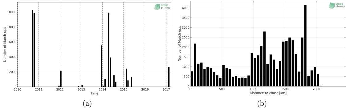
Figure 1: Number of match-ups between TSG (GOSUD-Sailing-ship) and SMOS L4 v2 Weekly (CATDS-CECOS-IFREMER) SSS as a function of time (a) and as function of the distance to coast (b) over the Tropical Atlantic Ocean Pi-MEP region and for the full satellite product period.
