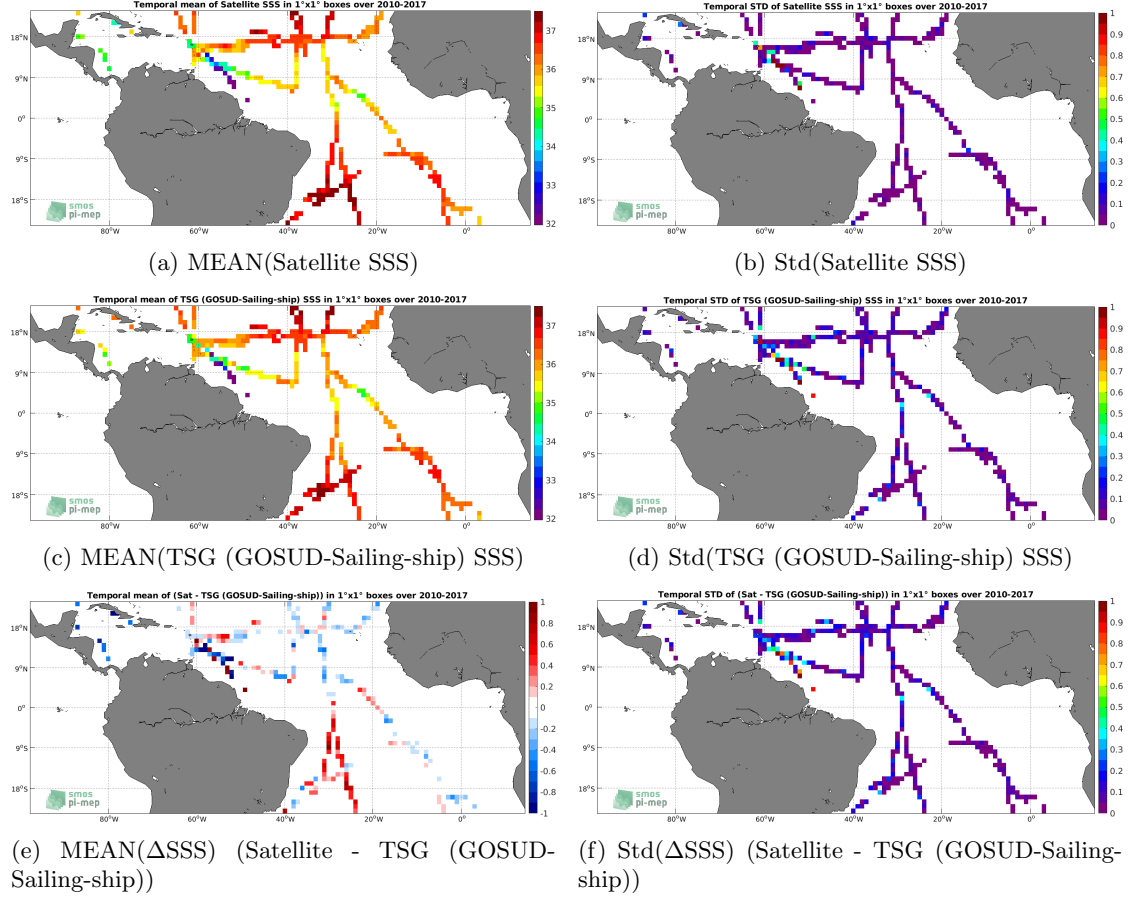
Figure 6: Temporal mean (left) and Std (right) of SSS from SMOS L4 v2 Weekly (CATDS-CECOS-IFREMER) (top), TSG (GOSUD-Sailing-ship) (middle), and of \Delta\text{SSS} (Satellite - TSG (GOSUD-Sailing-ship)). Only match-up pairs are used to generate these maps.
