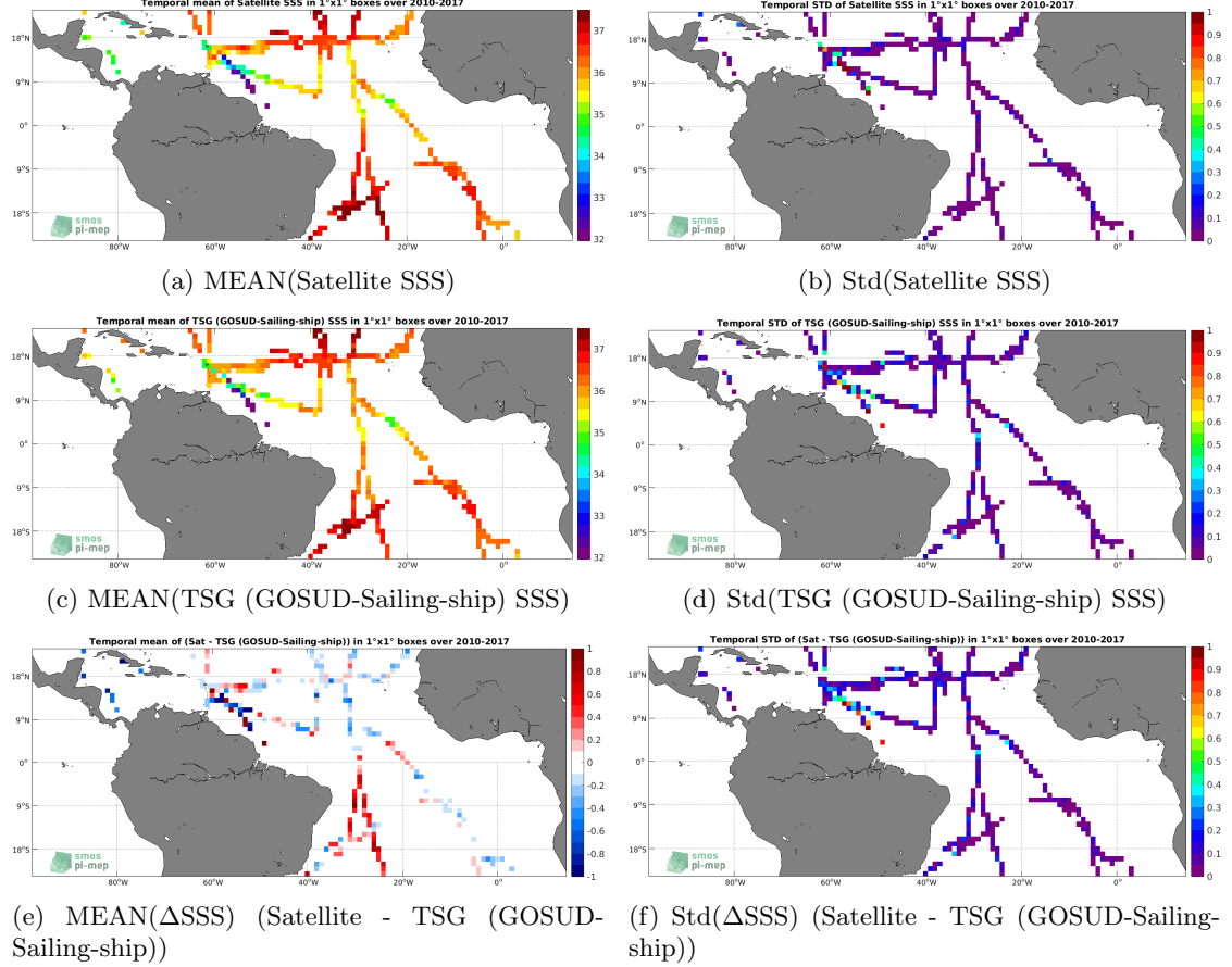
Figure 6: Temporal mean (left) and Std (right) of SSS from SMOS L4 v2 Weekly (CATDS-CECOS-IFREMER) (top), TSG (GOSUD-Sailing-ship) (middle), and of \Delta SSS (Satellite - TSG (GOSUD-Sailing-ship)). Only match-up pairs are used to generate these maps.
