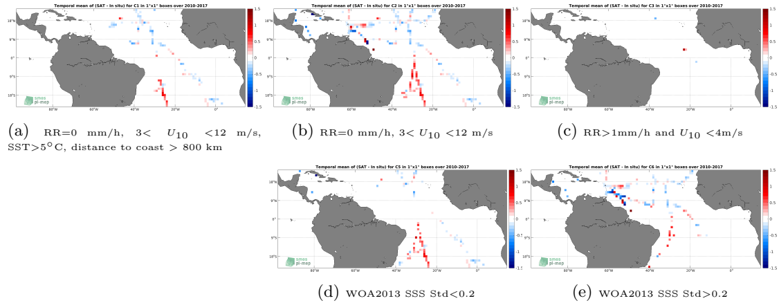
Figure 12: Temporal mean gridded over spatial boxes of size 1^\circ \times 1^\circ of \Delta SSS (SMOS L4 v2 Weekly (CATDS-CECOS-IFREMER) - TSG (GOSUD-Sailing-ship)) for 5 different subdatasets corresponding to: RR=0 mm/h, 3 < U_{10} < 12 m/s, SST >5^\circ\text{C} , distance to coast > 800 km (a), RR=0 mm/h, 3 < U_{10} < 12 m/s (b), RR >1 mm/h and U_{10} < 4 m/s (c), WOA2013 SSS Std <0.2 (d), WOA2013 SSS Std >0.2 (e).
