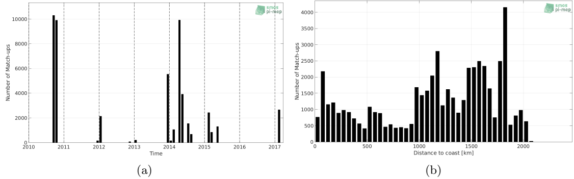
Figure 1: Number of match-ups between TSG-GOSUD-Sailing-ship and SMOS-L4-CATDS-CECOS-IFREMER-V2-WEEKLY-0.5DEG SSS as a function of time (a) and as function of the distance to coast (b) over the Tropical Atlantic Ocean Pi-MEP region and for the full satellite product period.
