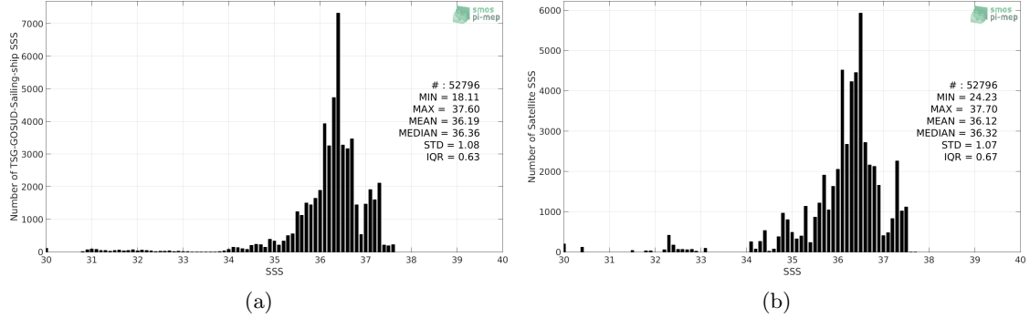
Figure 2: Histograms of SSS from TSG-GOSUD-Sailing-ship (a) and SMOS-L4-CATDS-CECOS-IFREMER-V2-WEEKLY-0.5DEG (b) considering all match-up pairs per bins of 0.1 over the Tropical Atlantic Ocean Pi-MEP region and for the full satellite product period.
