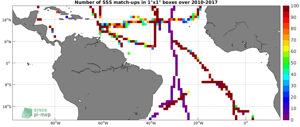
Figure 4: Number of SSS match-ups between TSG-GOSUD-Sailing-ship SSS and the SMOS-L4-CATDS-CECOS-IFREMER-V2-WEEKLY-0.5DEG SSS product for the Tropical Atlantic Ocean Pi-MEP region over 1^\circ \times 1^\circ boxes and for the full satellite product period.
