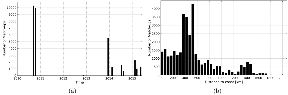
Figure 1: Number of match-ups between TSG-GOSUD-Sailing-ship and SMOS-L4-CATDS-CECOS-IFREMER-V2-WEEKLY-0.5DEG SSS as a function of time (a) and as function of the distance to coast (b) over the Tropical Atlantic Ocean Pi-MEP region and for the full satellite product period.
