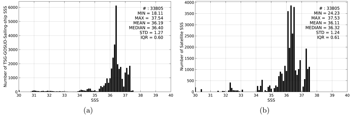
Figure 2: Histograms of SSS from TSG-GOSUD-Sailing-ship (a) and SMOS-L4-CATDS-CECOS-IFREMER-V2-WEEKLY-0.5DEG (b) considering all match-up pairs per bins of 0.1 over the Tropical Atlantic Ocean Pi-MEP region and for the full satellite product period.
