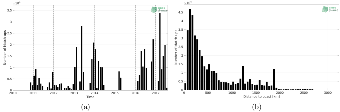
Figure 1: Number of match-ups between TSG (GOSUD-Research-vessel) and SMOS L4 v2 Weekly (CATDS-CECOS-IFREMER) SSS as a function of time (a) and as function of the distance to coast (b) over the Tropical Atlantic Ocean Pi-MEP region and for the full satellite product period.
