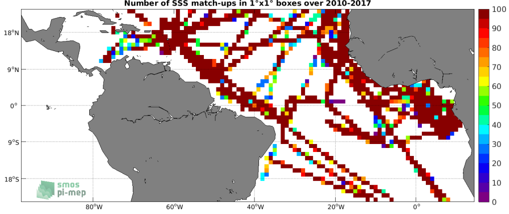
Figure 4: Number of SSS match-ups between TSG (GOSUD-Research-vessel) SSS and the SMOS L4 v2 Weekly (CATDS-CECOS-IFREMER) SSS product for the Tropical Atlantic Ocean Pi-MEP region over 1^\circ \times 1^\circ boxes and for the full satellite product period.
