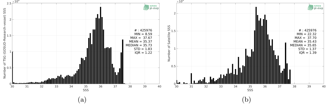
Figure 2: Histograms of SSS from TSG (GOSUD-Research-vessel) (a) and SMOS L4 v2 Weekly (CATDS-CECOS-IFREMER) (b) considering all match-up pairs per bins of 0.1 over the Tropical Atlantic Ocean Pi-MEP region and for the full satellite product period.
