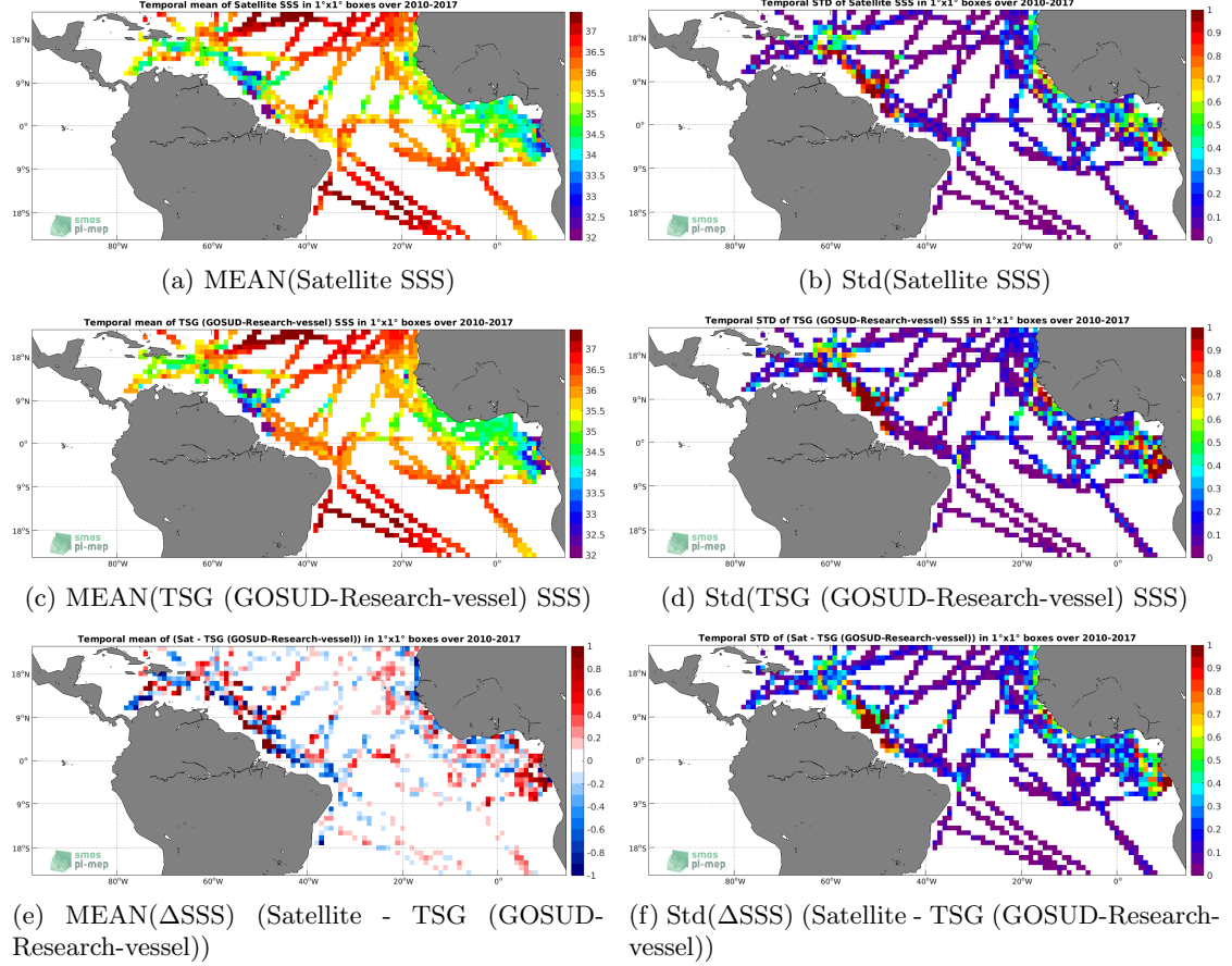
Figure 6: Temporal mean (left) and Std (right) of SSS from SMOS L4 v2 Weekly (CATDS-CECOS-IFREMER) (top), TSG (GOSUD-Research-vessel) (middle), and of \Delta SSS (Satellite - TSG (GOSUD-Research-vessel)). Only match-up pairs are used to generate these maps.
