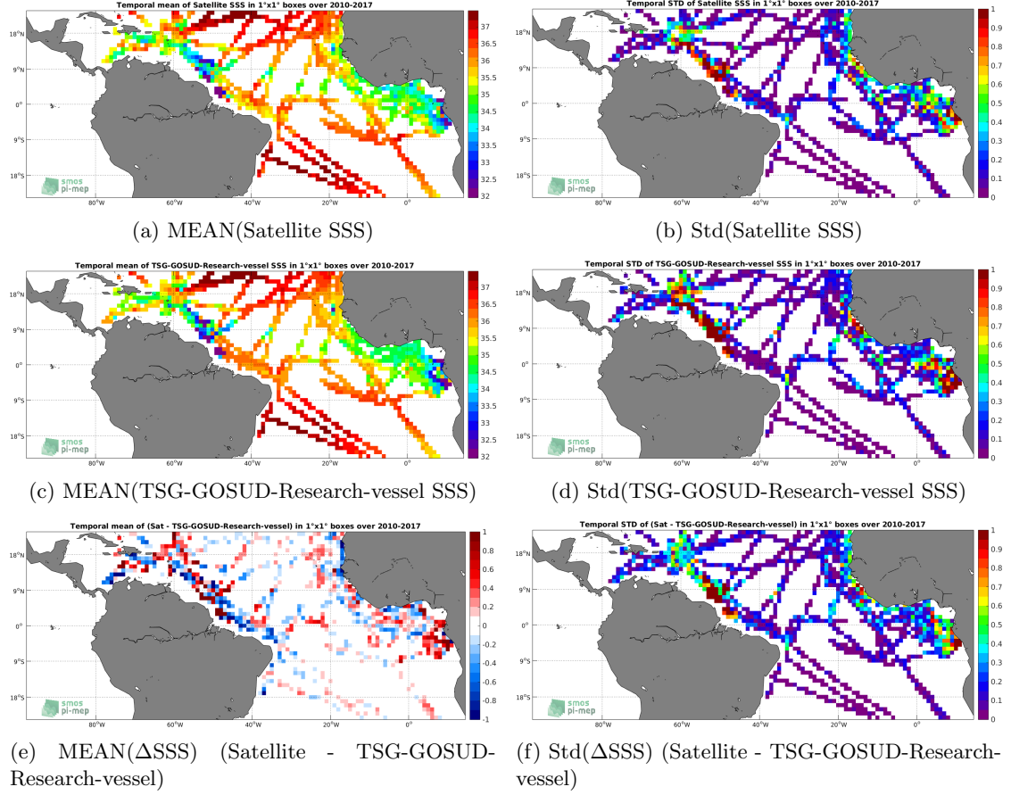
Figure 6: Temporal mean (left) and Std (right) of SSS from SMOS-L4-CATDS-CECOS-IFREMER-V2-WEEKLY-0.5DEG (top), TSG-GOSUD-Research-vessel (middle), and of \Delta\text{SSS} (Satellite - TSG-GOSUD-Research-vessel). Only match-up pairs are used to generate these maps.
