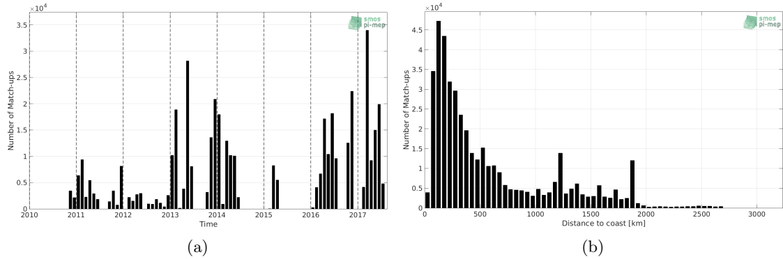
Figure 1: Number of match-ups between TSG-GOSUD-Research-vessel and SMOS-L4-CATDS-CECOS-IFREMER-V2-WEEKLY-0.5DEG SSS as a function of time (a) and as function of the distance to coast (b) over the Tropical Atlantic Ocean Pi-MEP region and for the full satellite product period.
