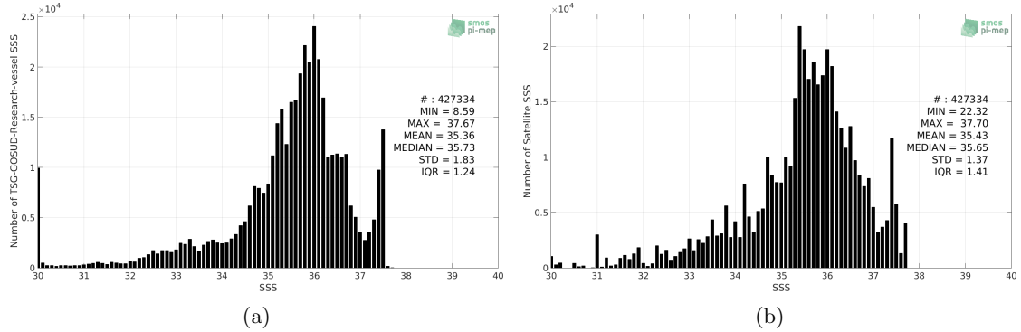
Figure 2: Histograms of SSS from TSG-GOSUD-Research-vessel (a) and SMOS-L4-CATDS-CECOS-IFREMER-V2-WEEKLY-0.5DEG (b) considering all match-up pairs per bins of 0.1 over the Tropical Atlantic Ocean Pi-MEP region and for the full satellite product period.
