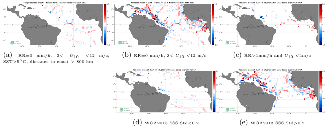
Figure 12: Temporal mean gridded over spatial boxes of size 1^\circ \times 1^\circ of \Delta SSS (SMOS-L4-CATDS-CECOS-IFREMER-V2-WEEKLY-0.5DEG - TSG-GOSUD-Research-vessel) for 5 different sub-datasets corresponding to: RR=0 mm/h, 3 < U_{10} < 12 m/s, SST>5°C, distance to coast > 800 km (a), RR=0 mm/h, 3 < U_{10} < 12 m/s (b), RR>1mm/h and U_{10} < 4 m/s (c), WOA2013 SSS Std<0.2 (d), WOA2013 SSS Std>0.2 (e).
