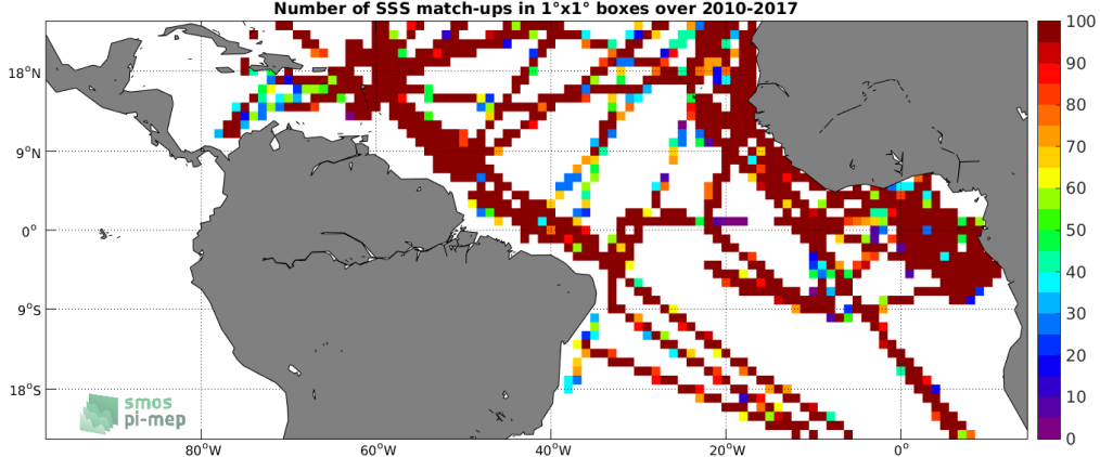
Figure 4: Number of SSS match-ups between TSG-GOSUD-Research-vessel SSS and the SMOS-L4-CATDS-CECOS-IFREMER-V2-WEEKLY-0.5DEG SSS product for the Tropical Atlantic Ocean Pi-MEP region over 1°x1° boxes and for the full satellite product period.
