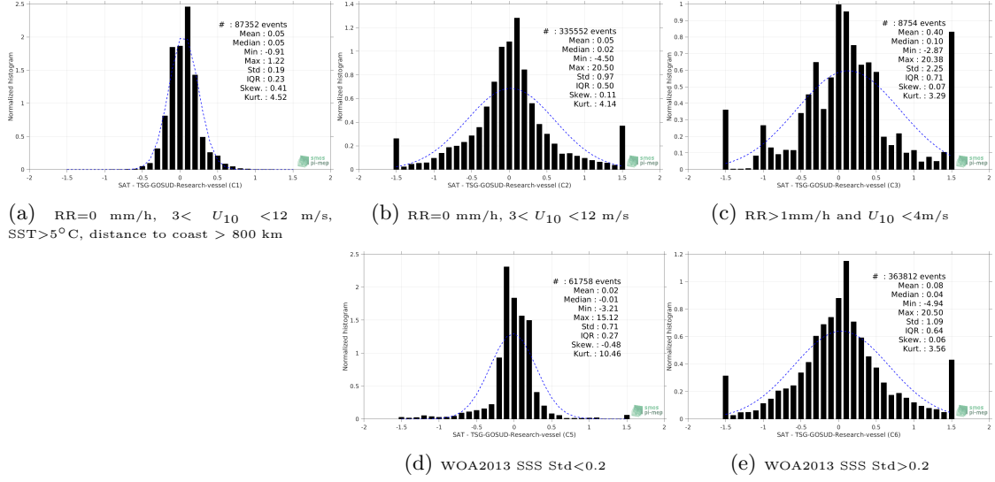
Figure 13: Normalized histogram of \Delta\text{SSS} (SMOS-L4-CATDS-CECOS-IFREMER-V2-WEEKLY-0.5DEG - TSG-GOSUD-Research-vessel) for 5 different subdatasets corresponding to: RR=0 mm/h, 3 < U_{10} < 12 m/s, SST > 5^{\circ}\text{C} , distance to coast > 800 km (a), RR=0 mm/h, 3 < U_{10} < 12 m/s (b), RR > 1\text{mm/h} and U_{10} < 4\text{m/s} (c), WOA2013 SSS Std < 0.2 (d), WOA2013 SSS Std > 0.2 (e).
