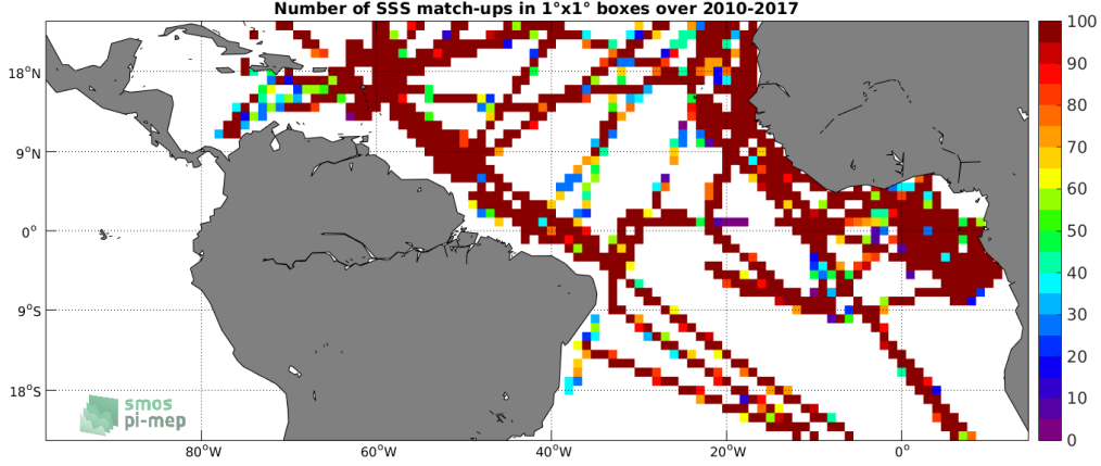
Figure 4: Number of SSS match-ups between TSG-GOSUD-Research-vessel SSS and the SMOS-L4-CATDS-CECOS-IFREMER-V2-WEEKLY-0.5DEG SSS product for the Tropical Atlantic Ocean Pi-MEP region over 1^\circ \times 1^\circ boxes and for the full satellite product period.
