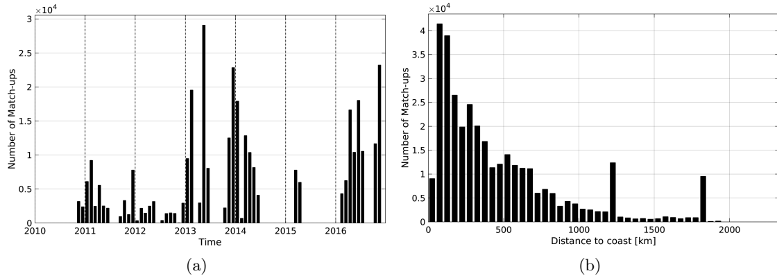
Figure 1: Number of match-ups between TSG-GOSUD-Research-vessel and SMOS-L4-CATDS-CECOS-IFREMER-V2-WEEKLY-0.5DEG SSS as a function of time (a) and as function of the distance to coast (b) over the Tropical Atlantic Ocean Pi-MEP region and for the full satellite product period.
