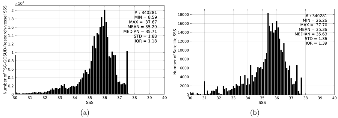
Figure 2: Histograms of SSS from TSG-GOSUD-Research-vessel (a) and SMOS-L4-CATDS-CECOS-IFREMER-V2-WEEKLY-0.5DEG (b) considering all match-up pairs per bins of 0.1 over the Tropical Atlantic Ocean Pi-MEP region and for the full satellite product period.
