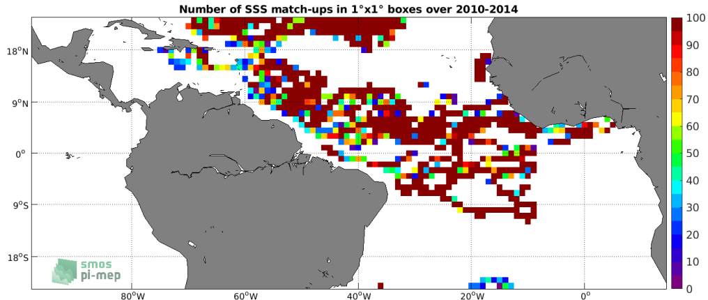
Figure 3: Number of SSS match-ups between Surface Drifters SSS and the SMOS L4 v2 Weekly (CATDS-CECOS-IFREMER) SSS product for the Tropical Atlantic Ocean Pi-MEP region over 1^\circ \times 1^\circ boxes and for the full satellite product period.
