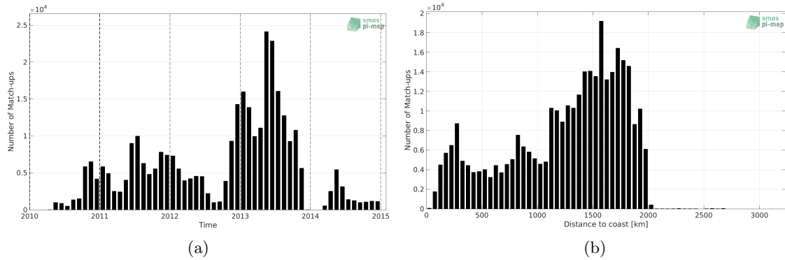
Figure 1: Number of match-ups between Surface drifters and SMOS L4 v2 Weekly (CATDS-CECOS-IFREMER) SSS as a function of time (a) and as function of the distance to coast (b) over the Tropical Atlantic Ocean Pi-MEP region and for the full satellite product period.
