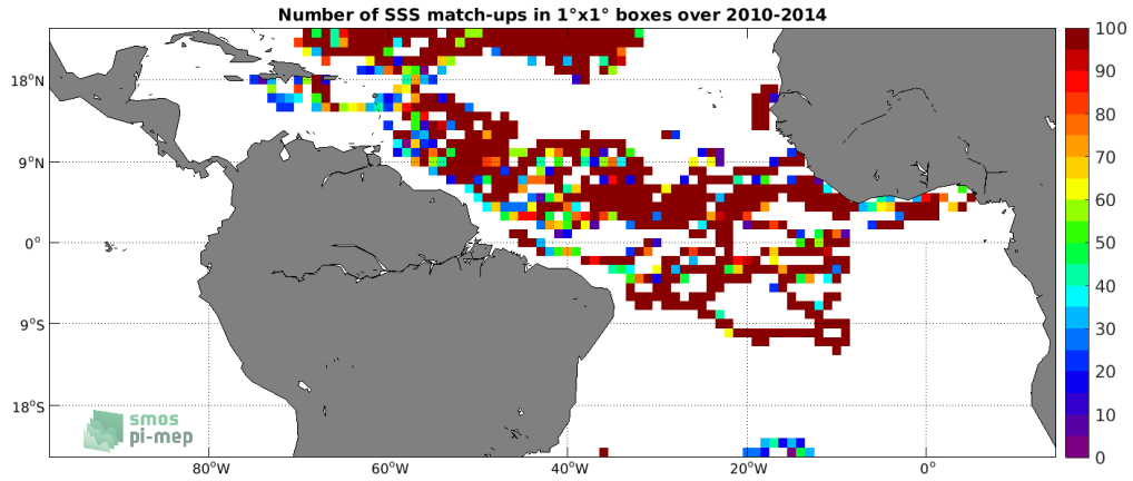
Figure 3: Number of SSS match-ups between Surface drifters SSS and the SMOS L4 v2 Weekly (CATDS-CECOS-IFREMER) SSS product for the Tropical Atlantic Ocean Pi-MEP region over 1°x1° boxes and for the full satellite product period.
