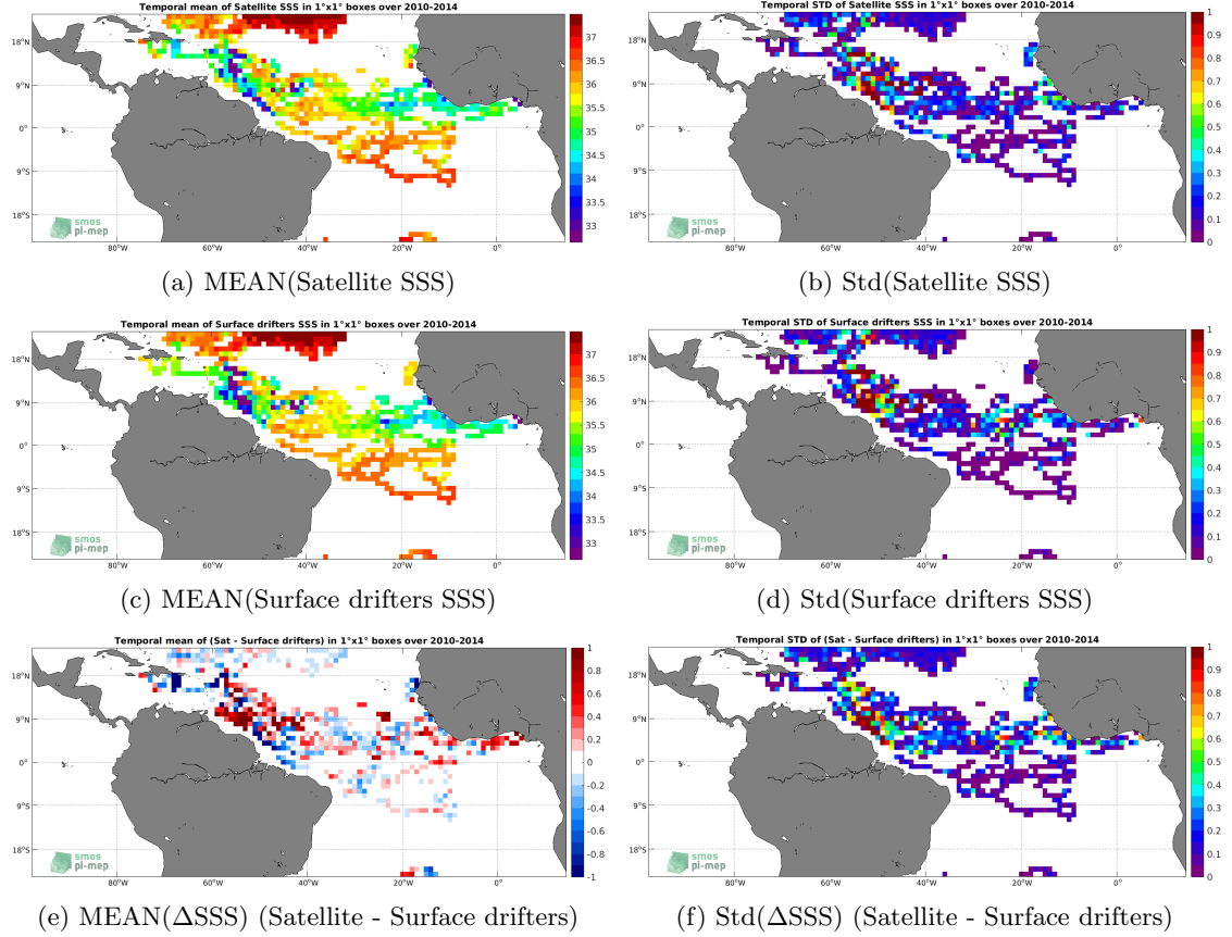
Figure 5: Temporal mean (left) and Std (right) of SSS from SMOS L4 v2 Weekly (CATDS-CECOS-IFREMER) (top), Surface drifters (middle), and of \Delta SSS (Satellite - Surface drifters). Only match-up pairs are used to generate these maps.
