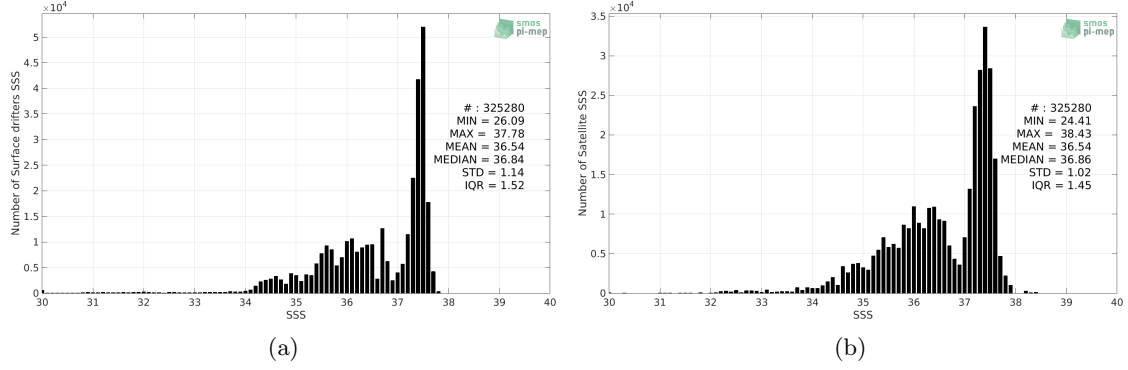
Figure 2: Histograms of SSS from Surface drifters (a) and SMOS L4 v2 Weekly (CATDS-CECOS-IFREMER) (b) considering all match-up pairs per bins of 0.1 over the Tropical Atlantic Ocean Pi-MEP region and for the full satellite product period.
