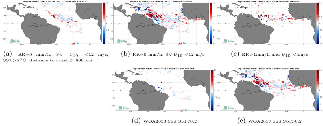
Figure 11: Temporal mean gridded over spatial boxes of size 1^{\circ}\times 1^{\circ} of \Delta\text{SSS} (SMOS-L4-CATDS-CECOS-IFREMER-V2-WEEKLY-0.5DEG - Surface drifters) for 5 different subdatasets corresponding to:RR=0 mm/h, 3 < U_{10} < 12 m/s, SST >5^{\circ}\text{C} , distance to coast > 800 km (a), RR=0 mm/h, 3 < U_{10} < 12 m/s (b), RR >1 mm/h and U_{10} < 4 m/s (c), WOA2013 SSS Std <0.2 (d), WOA2013 SSS Std >0.2 (e).
