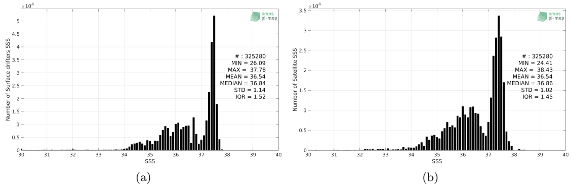
Figure 2: Histograms of SSS from Surface drifters (a) and SMOS-L4-CATDS-CECOS-IFREMER-V2-WEEKLY-0.5DEG (b) considering all match-up pairs per bins of 0.1 over the Tropical Atlantic Ocean Pi-MEP region and for the full satellite product period.
