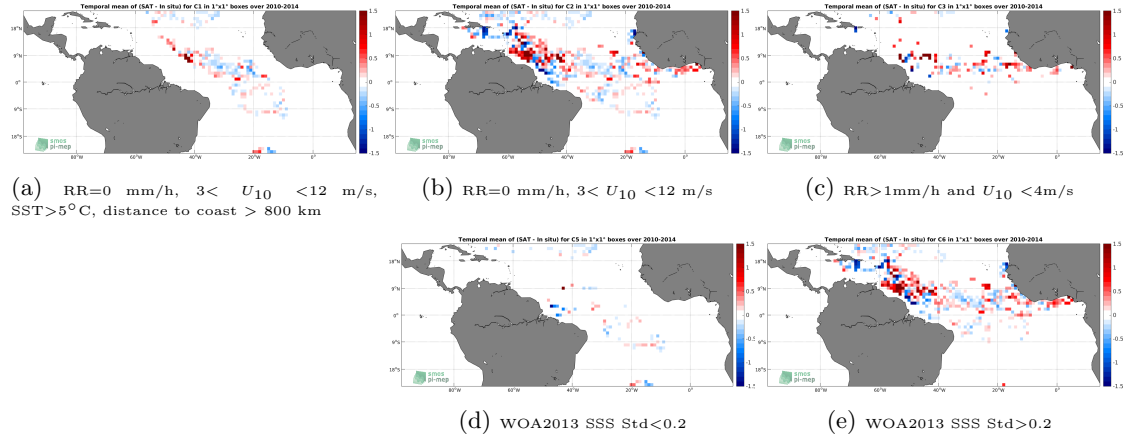
Figure 11: Temporal mean gridded over spatial boxes of size 1^\circ \times 1^\circ of \Delta SSS (SMOS-L4-CATDS-CECOS-IFREMER-V2-WEEKLY-0.5DEG - Surface drifters) for 5 different subdatasets corresponding to:RR=0 mm/h, 3 < U_{10} < 12 m/s, SST >5^\circ\text{C} , distance to coast > 800 km (a), RR=0 mm/h, 3 < U_{10} < 12 m/s (b), RR >1 mm/h and U_{10} < 4 m/s (c), WOA2013 SSS Std <0.2 (d), WOA2013 SSS Std >0.2 (e).
