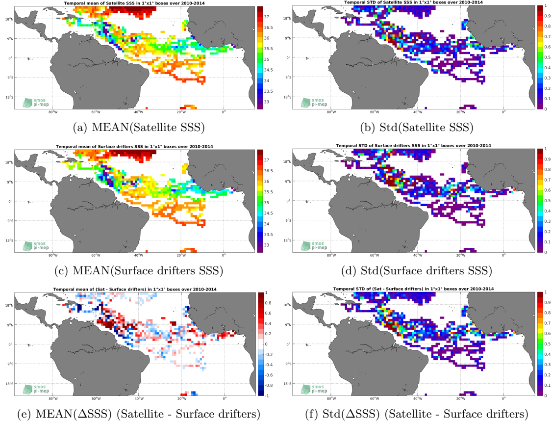
Figure 5: Temporal mean (left) and Std (right) of SSS from SMOS-L4-CATDS-CECOS-IFREMER-V2-WEEKLY-0.5DEG (top), Surface drifters (middle), and of \Delta SSS (Satellite - Surface drifters). Only match-up pairs are used to generate these maps.
