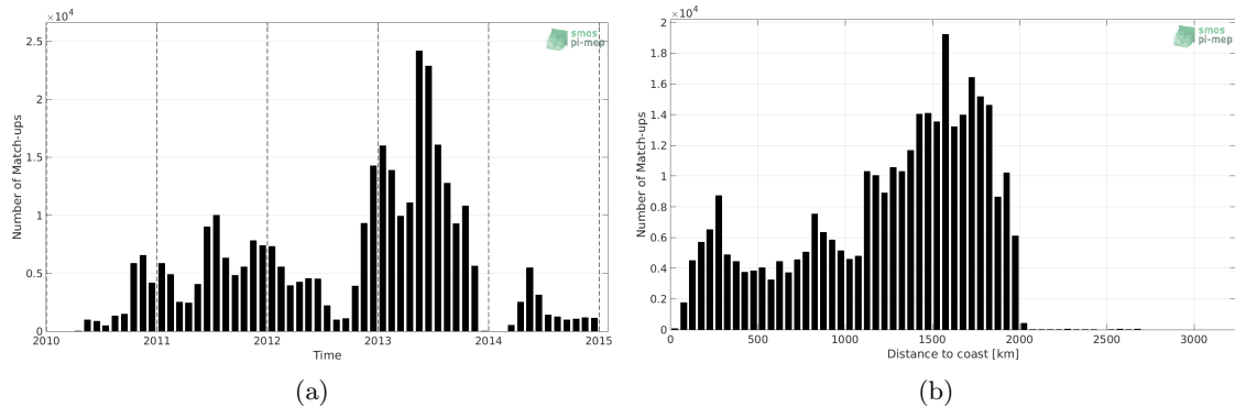
Figure 1: Number of match-ups between Surface drifters and SMOS-L4-CATDS-CECOS-IFREMER-V2-WEEKLY-0.5DEG SSS as a function of time (a) and as function of the distance to coast (b) over the Tropical Atlantic Ocean Pi-MEP region and for the full satellite product period.
