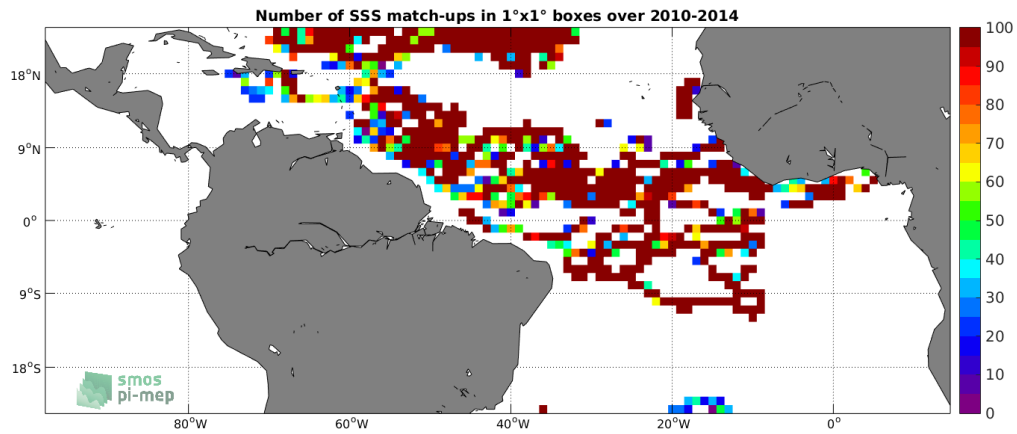
Figure 3: Number of SSS match-ups between Surface drifters SSS and the SMOS-L4-CATDS-CECOS-IFREMER-V2-WEEKLY-0.5DEG SSS product for the Tropical Atlantic Ocean Pi-MEP region over 1°x1° boxes and for the full satellite product period.
