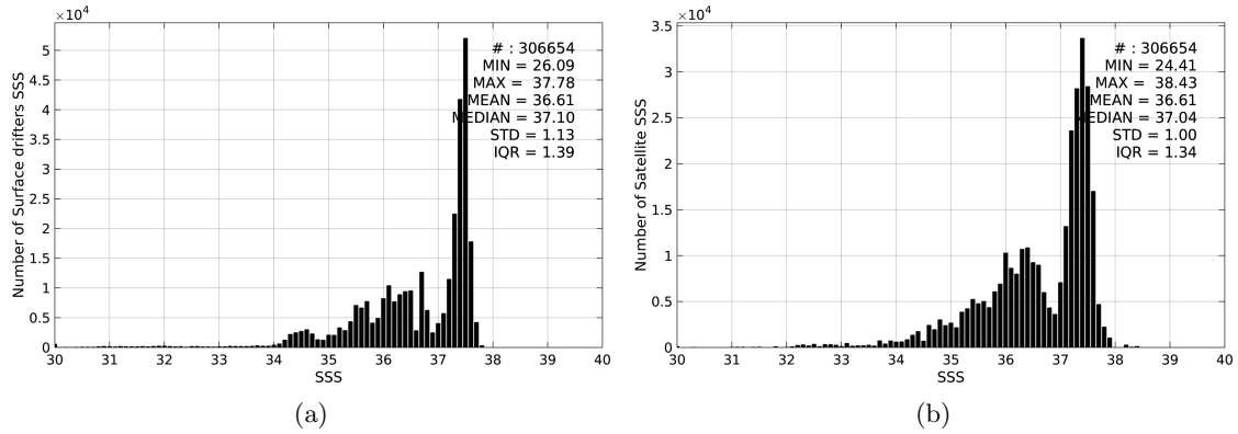
Figure 2: Histograms of SSS from Surface drifters (a) and SMOS-L4-CATDS-CECOS-IFREMER-V2-WEEKLY-0.5DEG (b) considering all match-up pairs per bins of 0.1 over the Tropical Atlantic Ocean Pi-MEP region and for the full satellite product period.
