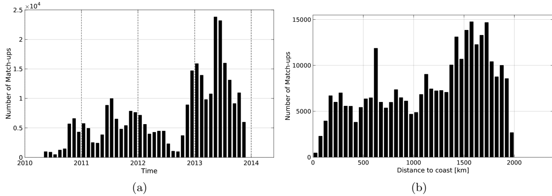
Figure 1: Number of match-ups between Surface drifters and SMOS-L4-CATDS-CECOS-IFREMER-V2-WEEKLY-0.5DEG SSS as a function of time (a) and as function of the distance to coast (b) over the Tropical Atlantic Ocean Pi-MEP region and for the full satellite product period.
