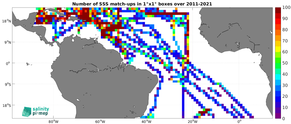
Figure 5: Number of SSS match-ups between TSG (SAMOS) SSS and the SMOS SSS L4 v2 - Daily (BEC) SSS product for the Tropical Atlantic Ocean Pi-MEP region over 1^\circ \times 1^\circ boxes and for the full satellite product period.
