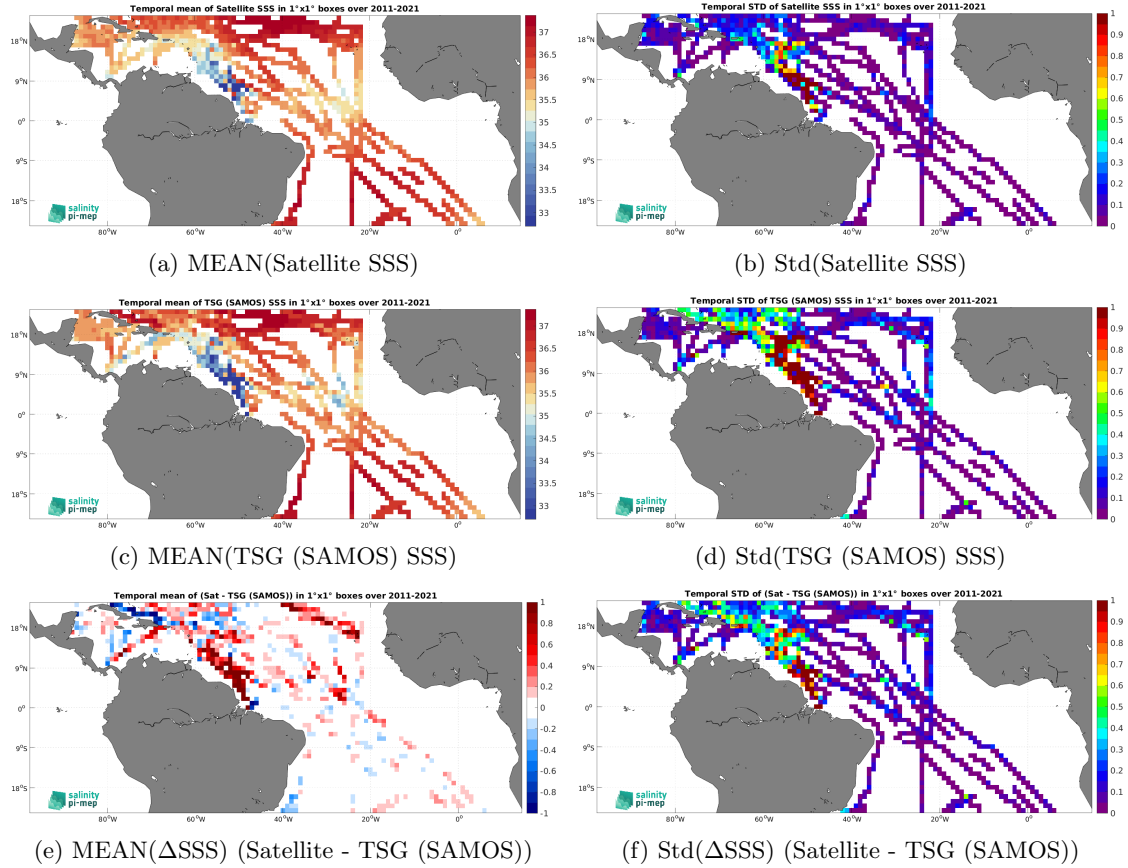
Figure 7: Temporal mean (left) and Std (right) of SSS from SMOS SSS L4 v2 - Daily (BEC) (top), TSG (SAMOS) (middle), and of \Delta SSS (Satellite - TSG (SAMOS)). Only match-up pairs are used to generate these maps.
