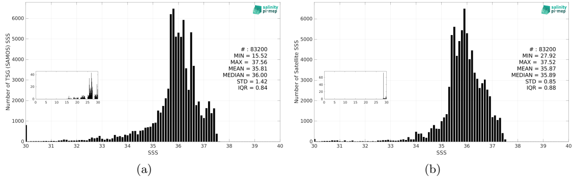
Figure 3: Histograms of SSS from TSG (SAMOS) (a) and SMOS SSS L4 v2 - Daily (BEC) (b) considering all match-up pairs per bins of 0.1 over the Tropical Atlantic Ocean Pi-MEP region and for the full satellite product period.
