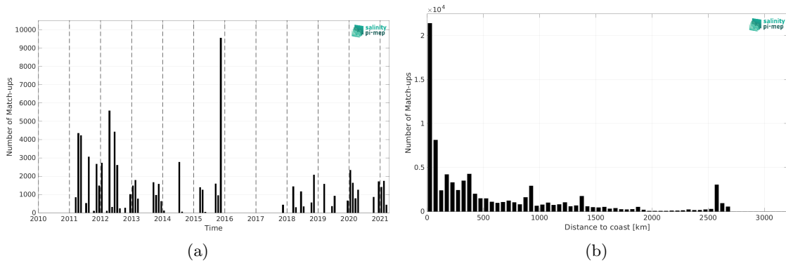
Figure 2: Number of match-ups between TSG (SAMOS) and SMOS SSS L4 v2 - Daily (BEC) SSS as a function of time (a) and as function of the distance to coast (b) over the Tropical Atlantic Ocean Pi-MEP region and for the full satellite product period.
