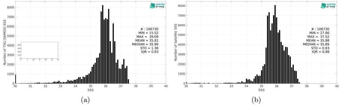
Figure 2: Histograms of SSS from TSG (SAMOS) (a) and SMOS SSS L4 v2 - Daily (BEC) (b) considering all match-up pairs per bins of 0.1 over the Tropical Atlantic Ocean Pi-MEP region and for the full satellite product period.
