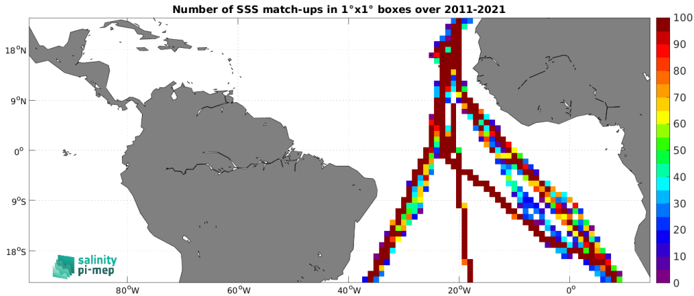
Figure 5: Number of SSS match-ups between TSG (Polarstern) SSS and the SMOS SSS L4 v2 - Daily (BEC) SSS product for the Tropical Atlantic Ocean Pi-MEP region over 1^\circ \times 1^\circ boxes and for the full satellite product period.
