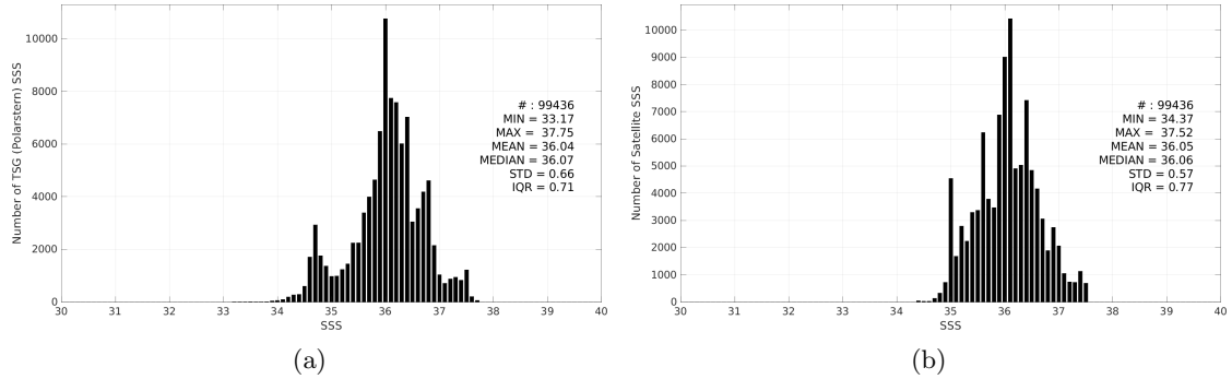
Figure 3: Histograms of SSS from TSG (Polarstern) (a) and SMOS SSS L4 v2 - Daily (BEC) (b) considering all match-up pairs per bins of 0.1 over the Tropical Atlantic Ocean Pi-MEP region and for the full satellite product period.
