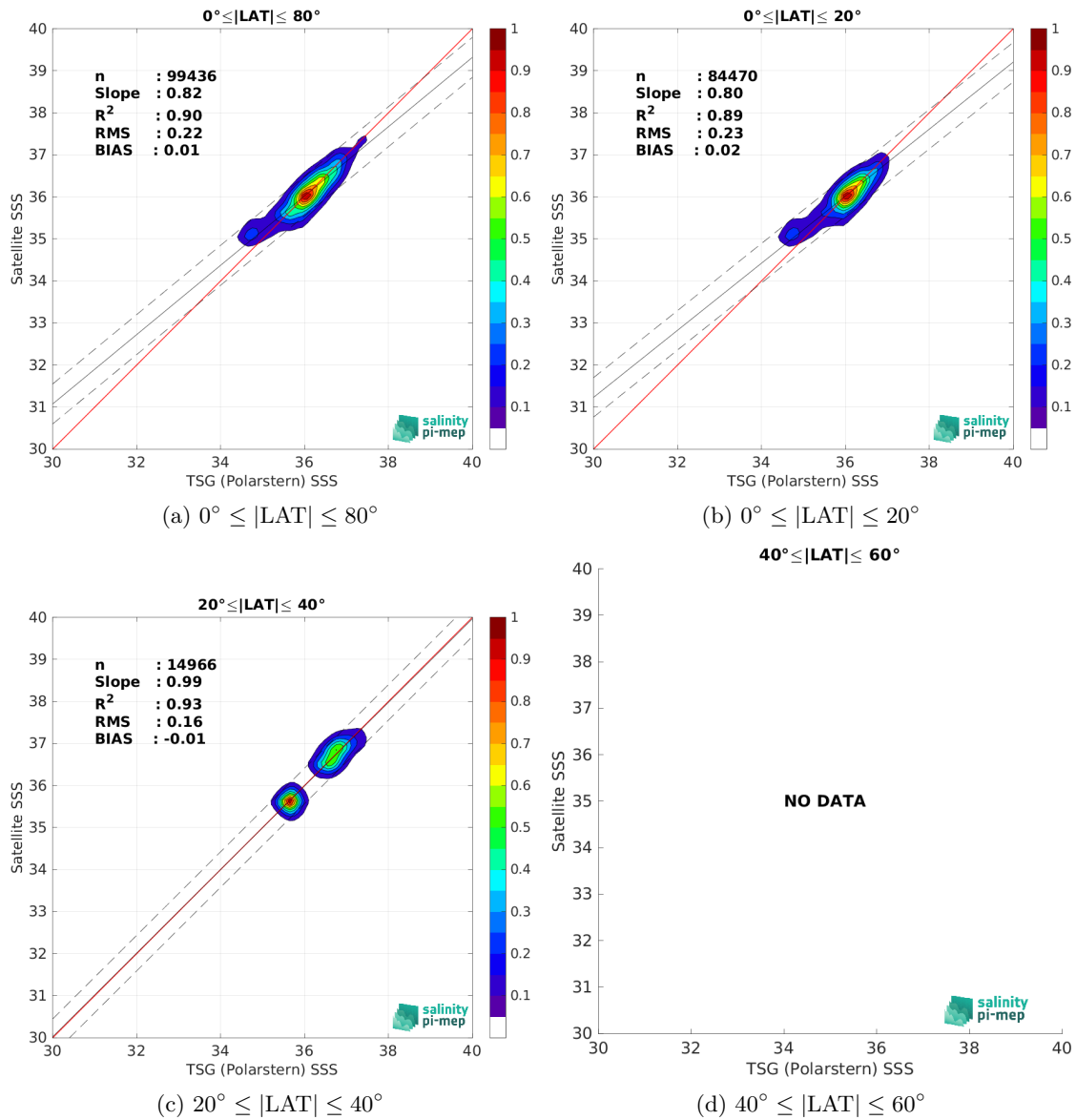
Figure 10: Contour maps of the concentration of SMOS SSS L4 v2 - Daily (BEC) SSS (y-axis) versus TSG (Polarstern) SSS (x-axis) at match-up pairs for different latitude bands. For each plot, the red line shows x=y . The black thin and dashed lines indicate a linear fit through the data cloud and the \pm 95\% confidence levels, respectively. The number match-up pairs n , the slope and R^2 coefficient of the linear fit, the root mean square (RMS) and the mean bias between satellite and in situ data are indicated for each latitude band in each plots.
