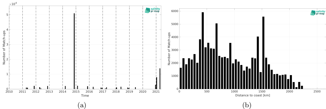
Figure 2: Number of match-ups between TSG (Polarstern) and SMOS SSS L4 v2 - Daily (BEC) SSS as a function of time (a) and as function of the distance to coast (b) over the Tropical Atlantic Ocean Pi-MEP region and for the full satellite product period.
