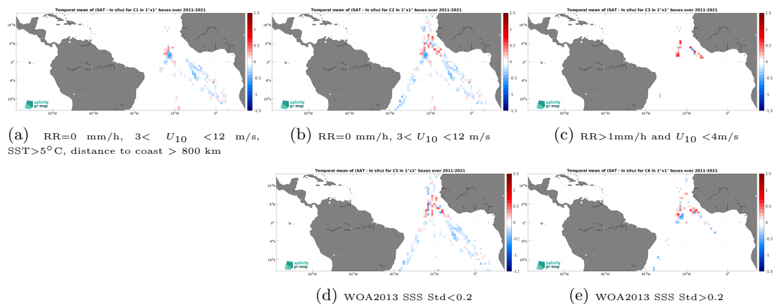
Figure 14: Temporal mean gridded over spatial boxes of size 1^\circ \times 1^\circ of \Delta\text{SSS} (SMOS SSS L4 v2 - Daily (BEC) - TSG (Polarstern)) for 5 different subdatasets corresponding to:RR=0 mm/h, 3 < U_{10} < 12 m/s, SST >5^\circ\text{C} , distance to coast > 800 km (a), RR=0 mm/h, 3 < U_{10} < 12 m/s (b), RR >1 mm/h and U_{10} < 4 m/s (c), WOA2013 SSS Std <0.2 (d), WOA2013 SSS Std >0.2 (e).
