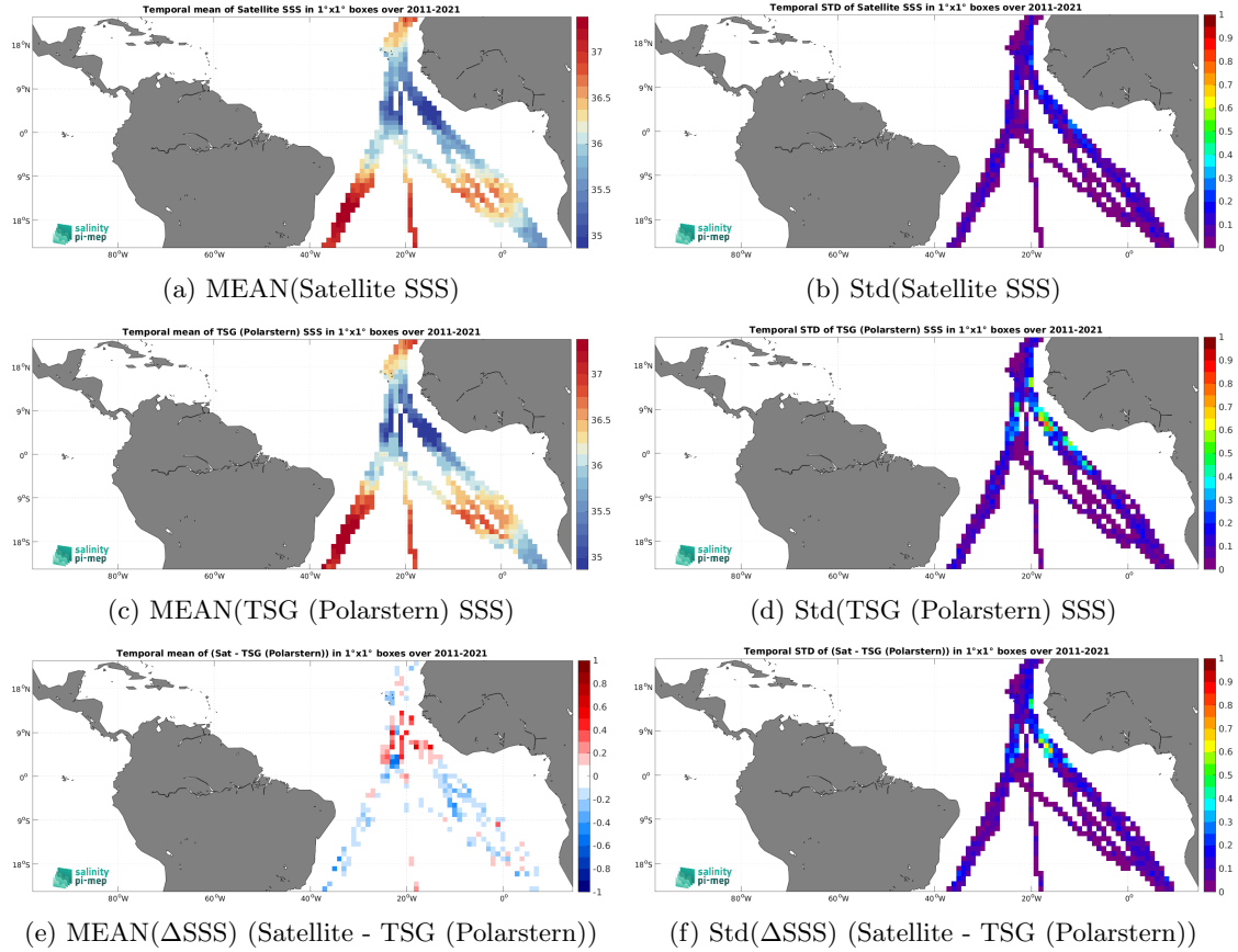
Figure 7: Temporal mean (left) and Std (right) of SSS from SMOS SSS L4 v2 - Daily (BEC) (top), TSG (Polarstern) (middle), and of \Delta\text{SSS}(\text{Satellite} - \text{TSG}(\text{Polarstern})) . Only match-up pairs are used to generate these maps.
